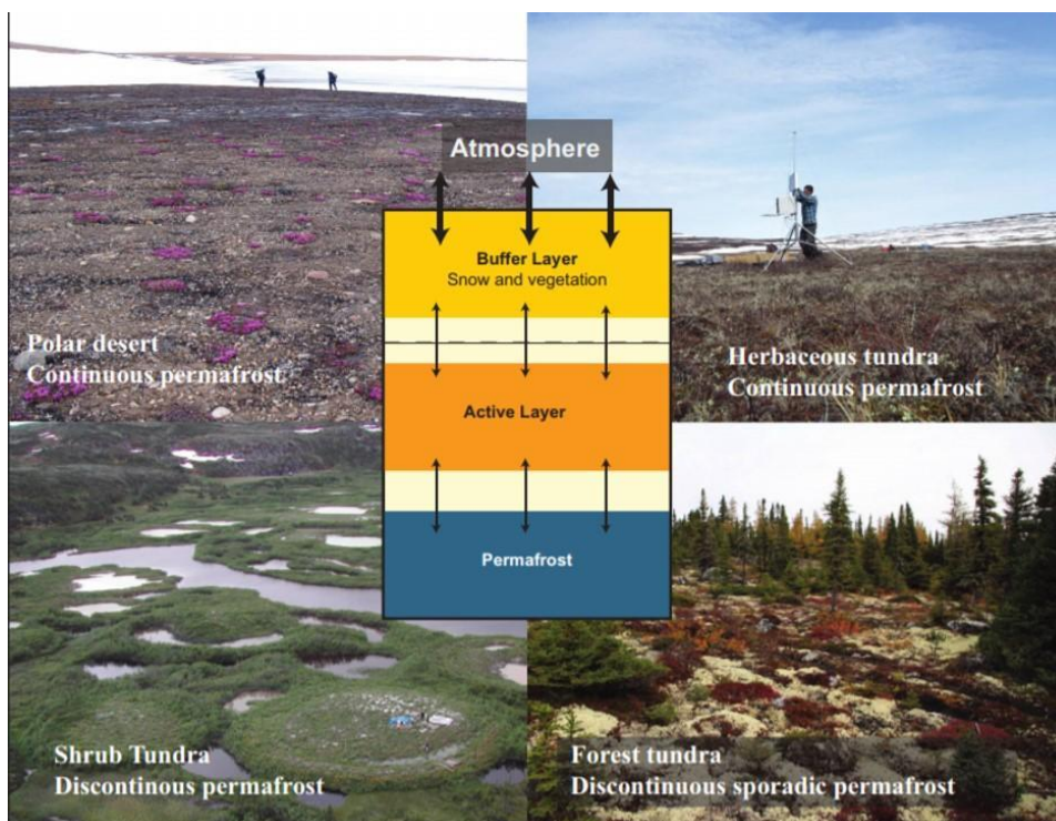
Figure 4.6: (Fig. 4 in Vincent et al., 2017): The three-layer model applied to natural landscapes. As illustrated here, the buffer layer varies greatly in its geometry (thickness), albedo, and other physical properties, both within and between landscapes, and as a function of vegetation type and season. The arrows indicate exchanges of heat, water, and gases and the white bands indicate interface zones. Upper left: Ward Hunt Island, Nunavut; upper right: Daring Lake, Northwest Territories; lower left: BGR valley, Nunavik; lower right: Umiujaq region, Nunavik.
