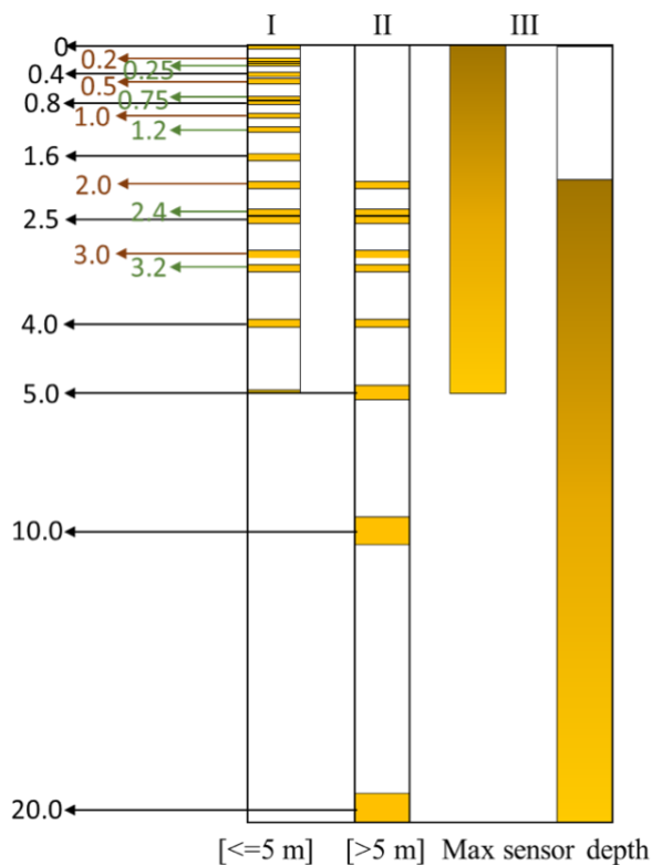
Figure 4.4: Discrete depths are provided small-scaled in shallower depths and larger scaled in deeper depths. In deep boreholes (Group II, >5 m depth), <1.5-2 m measurements were discarded due to their inaccuracy due to large borehole diameter and air or artificial infillings. In Group III, temperature data are interpolated for shallow and deep temperature profiles down to the maximum sensor depth. Also here, the upper 1.5-2 m temperature measurements of deep boreholes are discarded.
