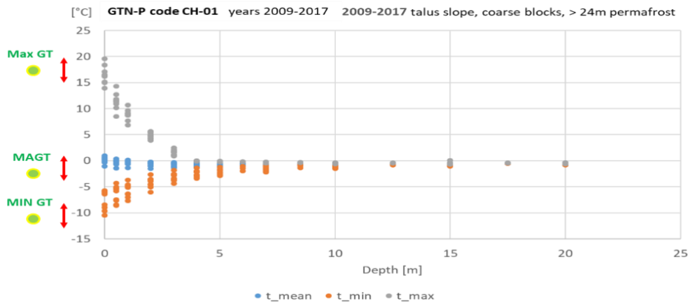
Figure 4.8: High inter-annual variability of MAGT, min annual GT and max annual GT in mountain permafrost
