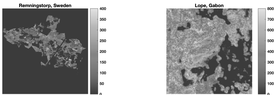
Figure 3-7: AGB maps with a resolution of 20 m × 20 m derived from ALS data acquired over the test sites Remningstorp, Sweden, and Lope, Gabon.
