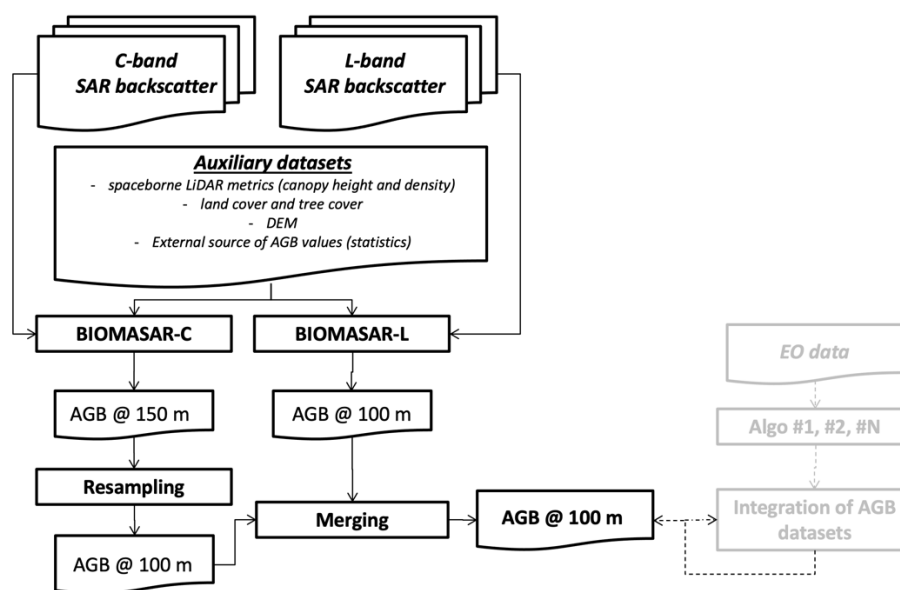
Figure 3-4: Functional dependencies of datasets and approaches forming the CCI BIOMASS global biomass retrieval algorithm. The shaded part of the flowchart represents potential improvements following the implementation of additional retrieval techniques.
