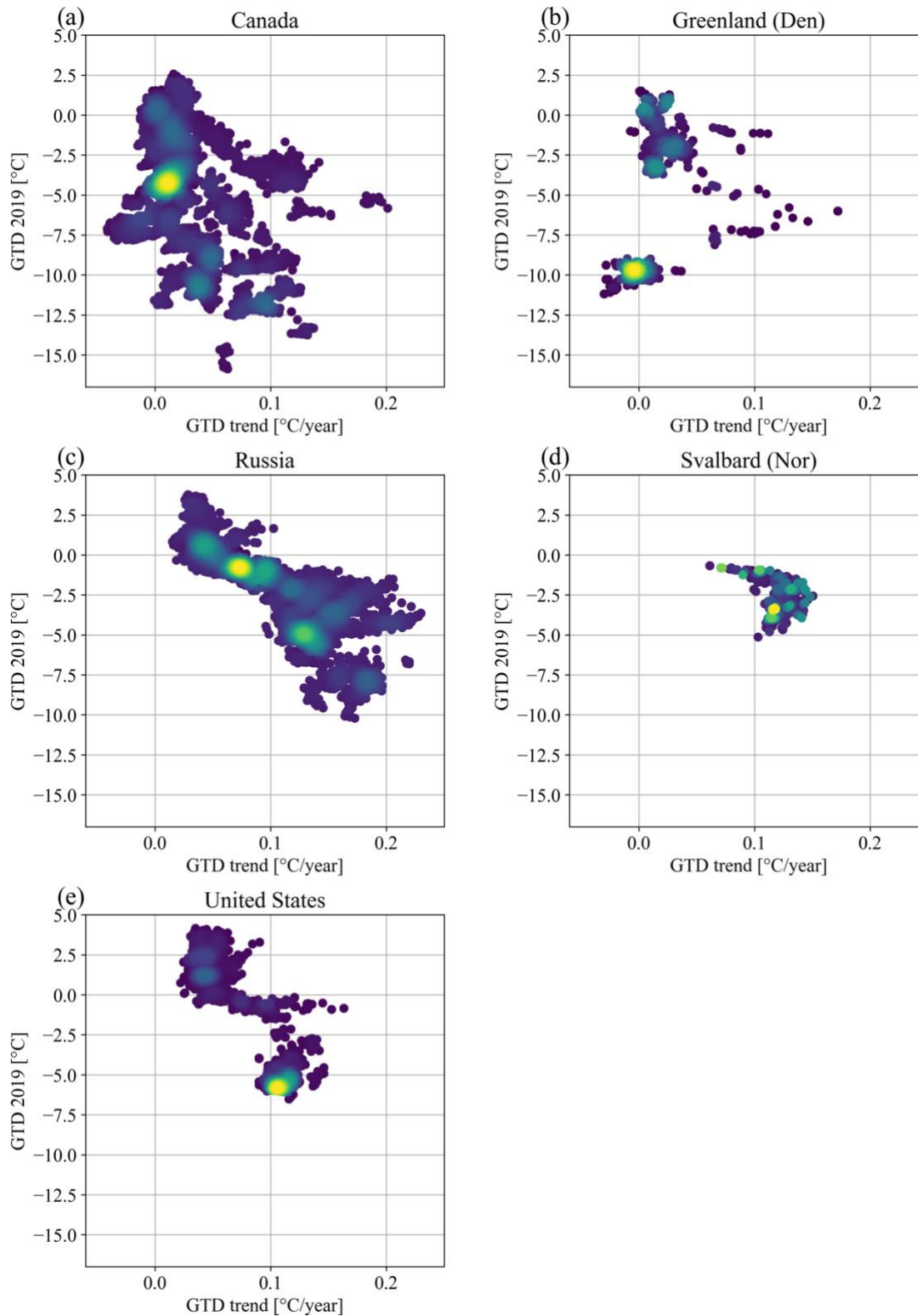
Figure 11: Scatterplots of trend versus 2019 status for Ground temperature at 2 m depth separated by region. Each point represents the average for a distinct object within human impacted areas as mapped with Sentinel-1 and -2. Calculations are based on CRDPv2. Modified from Bartsch et al. (2021)
