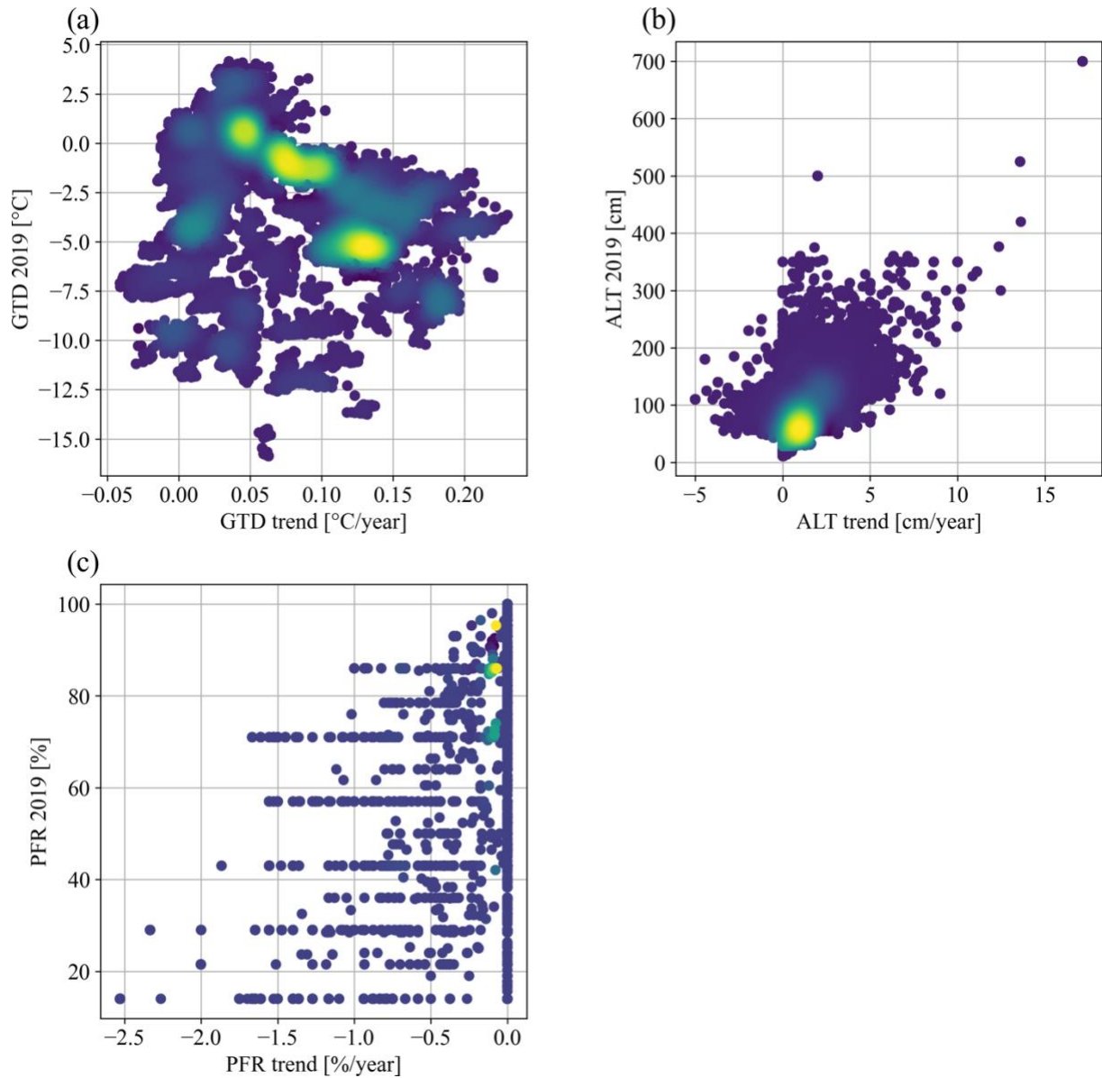
Figure 10: Scatterplots of trend versus 2019 status for a) Ground temperature at 2 m depth, b) Active layer thickness and c) Permafrost fraction. Each point represents the average for a distinct object within human impacted areas as mapped with Sentinel-1 and -2. Calculations are based on CRDPv2. Source: Bartsch et al. (2021)
