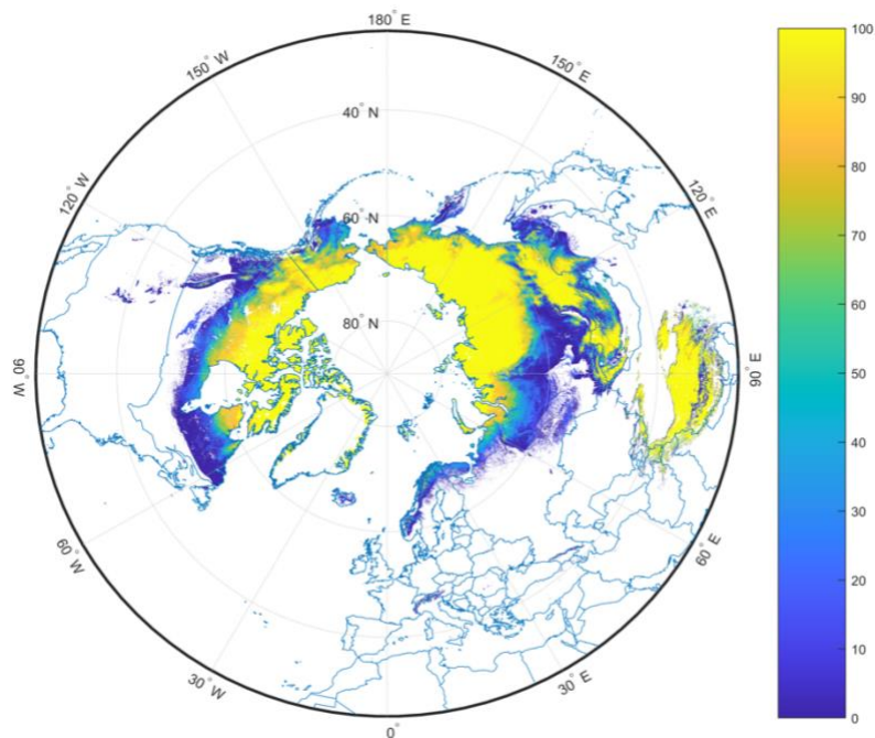
Figure 3: Example of Active Layer Thickness for 2019 (from 0 to 100%, colour axis).
