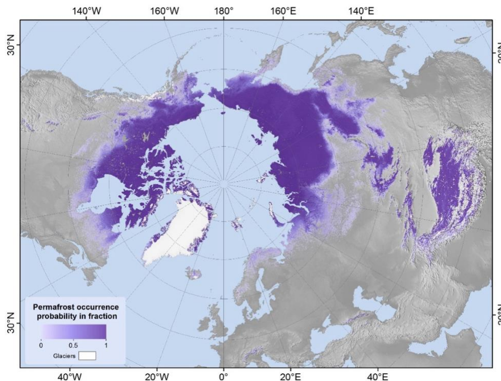
Figure 5: Example of Permafrost extent (fraction) for 2015
