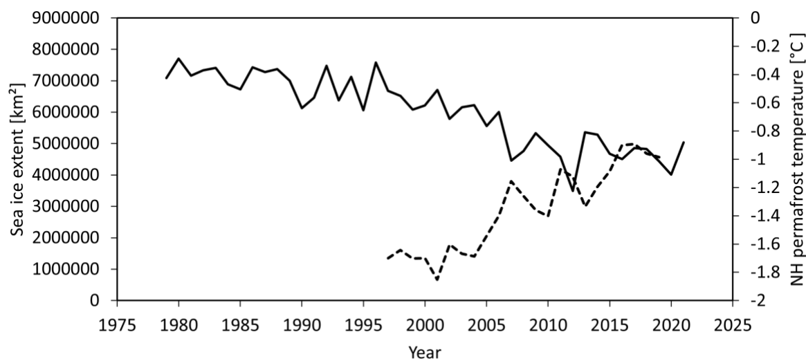
Figure 9: Northern hemisphere (NH) permafrost temperature change at 2 m depth (dashed line; source transient modelling using landsurface temperature (reanalyses data and near infrared (MODIS, 1 km); CryoGRID; Permafrost_cci v3 (CRDPv2), compared to sea ice extent for September (solid line; sea ice concentration data from 1979 to 2021 were obtained from https://www.meerisportal.de/grant/REKLIM-2013-04 , Spreen et al. (2008)). Source: Bartsch et al. (2023).
