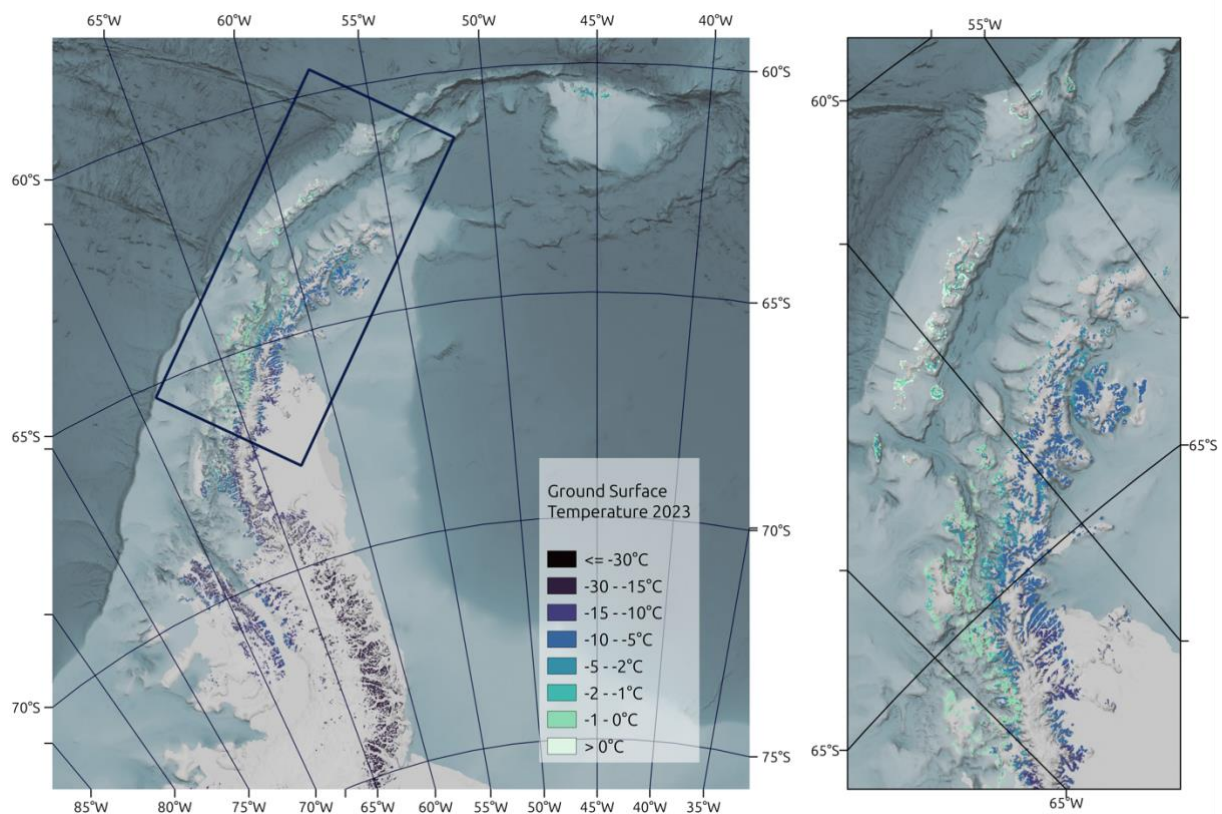
Figure 2: Example of Mean Annual Ground Surface Temperature in 2023 for Antarctica (CRDPv4).
