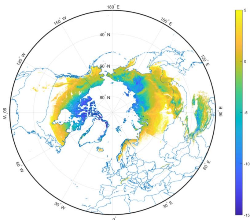
Figure 1: Example of Northern Hemisphere Mean Annual Ground Temperature at 2 m depth in 2019 (in °C, colour axis).
