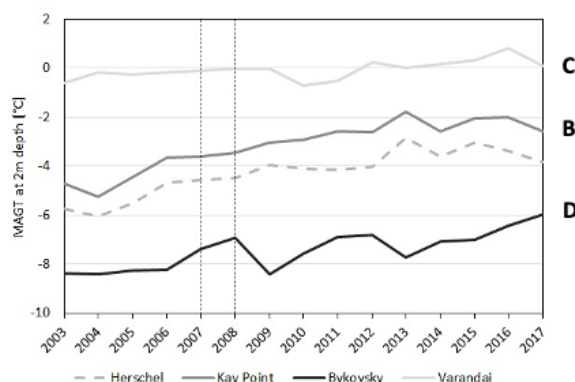
Figure 8: Erosion rate retrieval summary from Bartsch et al. (2020). Most sites show increased recent rates (left) as well as increasing ground temperatures (right, source CRDPv0). GlobPermafrost product: Landsat based rates. L-band SAR: PALSAR and PALSAR2.
