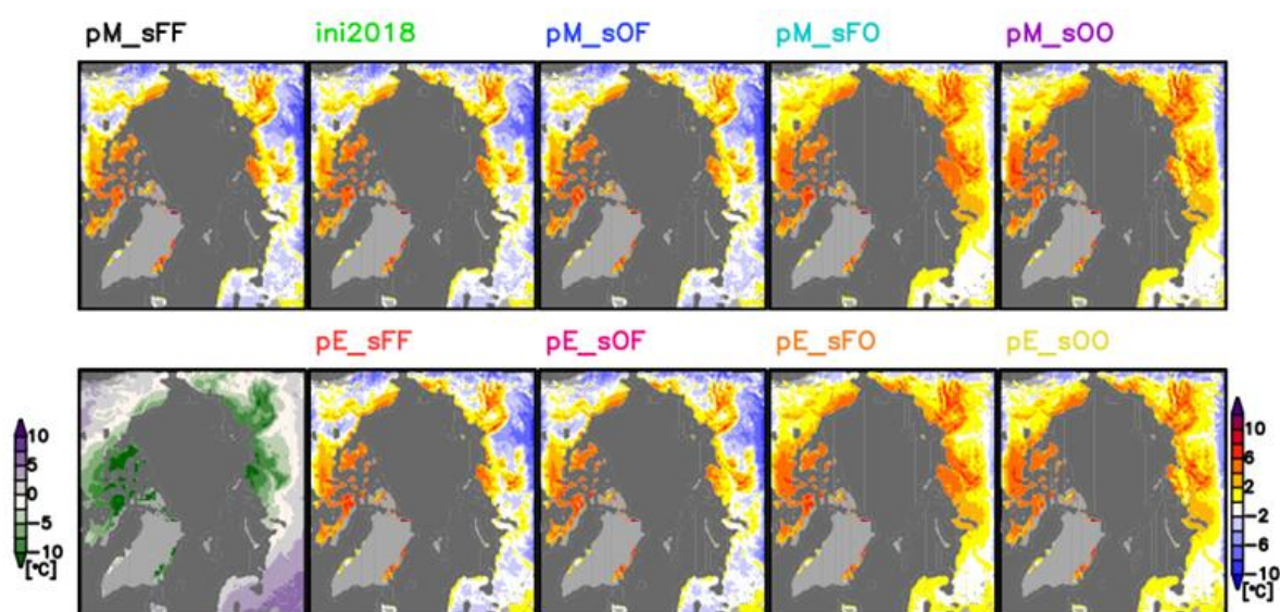
Figure 6: Mean annual ground temperature at 1m depth, averaged over 2003-2019, from CCI+ Permafrost product (lower left panel) and difference to HIRHAM-CLM model runs (model run minus CCI+Permafrost). For abbreviations see [RD-4].
