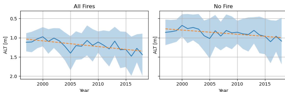
Figure 7: Mean (line), standard deviation (shading) and trend of mean (orange dashed line) of modelled active layer thickness (ALT) in burned and unburned regions in Transect T3 Alaska. (for details see [RD-4]).
