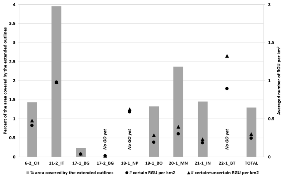
Figure 7. The density of the rock glaciers (number of RGU per km 2 and percentage of the area covered by rock glaciers according to the mapped extended GOs). The area numbers follow the standard format defined in the PSD [RD-2] and the PUG [RD-9]. See Figure 1 for geographical reference.
