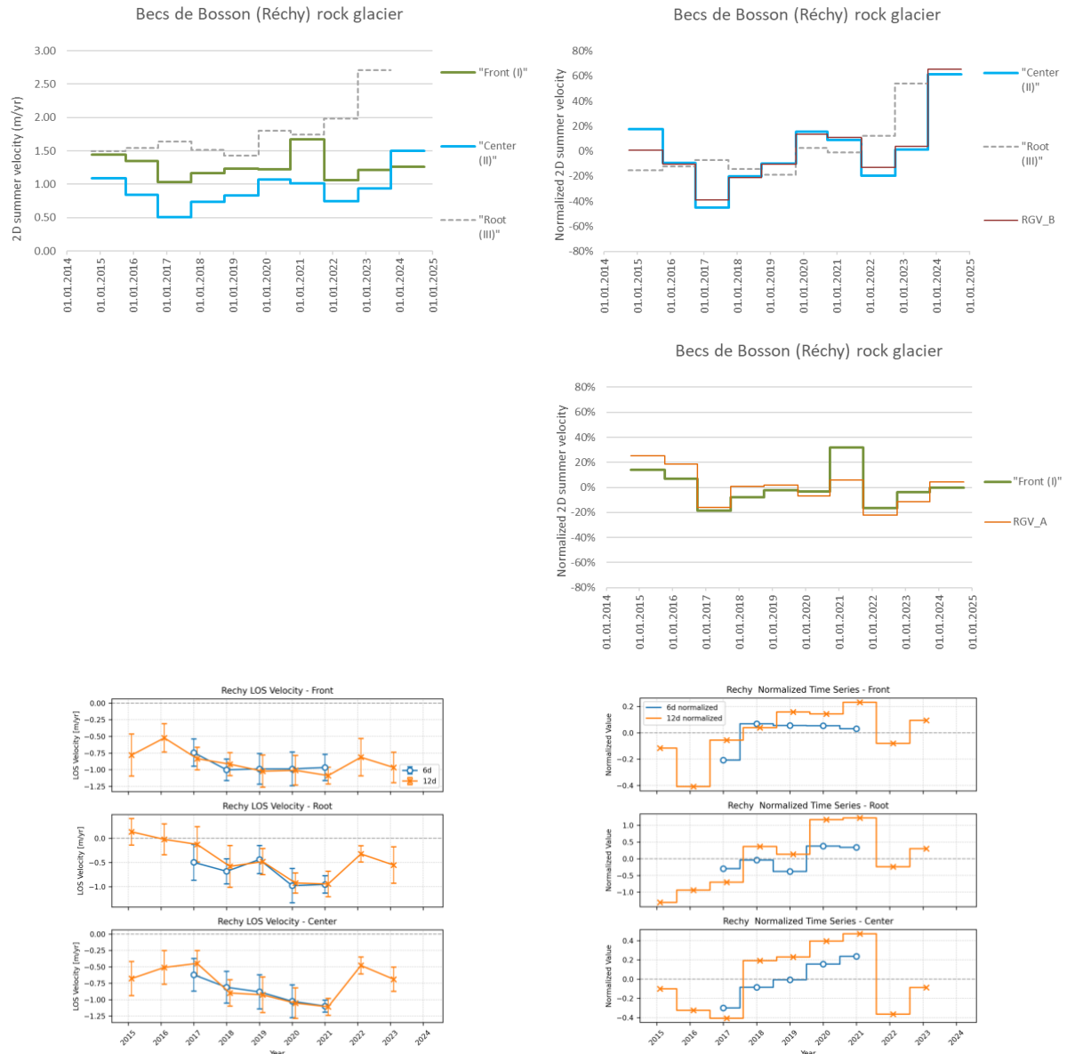
Figure 16. Comparison between available GNSS-RGV data (upper graphs) and Permafrost_cci InSAR-RGV (lower graphs) on Réchy rock glacier. Left: m/yr velocity time series. Right: Relative velocity changes.
