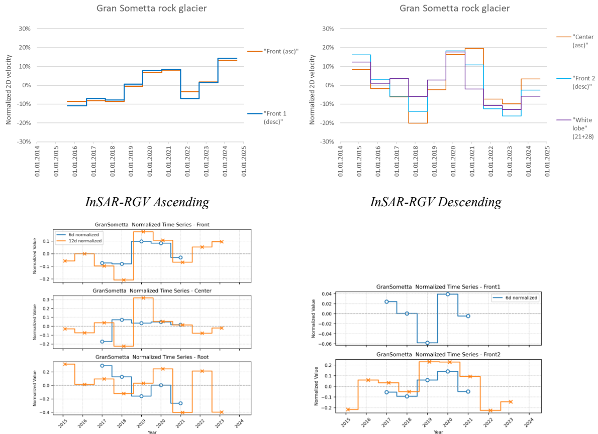
Figure 18. Comparison between available GNSS-RGV data (upper graph) and Permafrost_cci InSAR-RGV (lower graphs) on Gran Sometta rock glacier.
