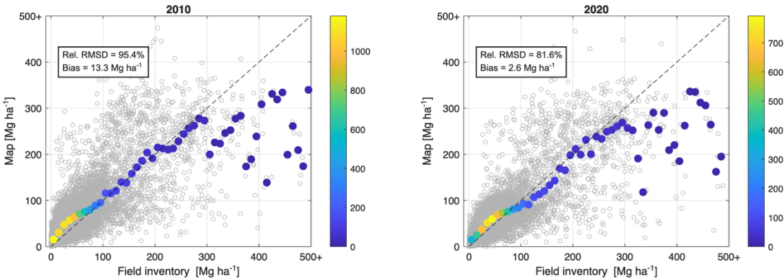
Figure 3-5: Scatterplots of average AGB from field inventory data (x axis) and corresponding values from the AGB map (y axis) using a 0.1° (i.e., 10 km) grid for the years 2010 and 2020 (year 7, V7.0). In each scatterplot, the coloured circles represent the average map value for binned reference AGB (10 Mg ha -1 wide intervals). The colour represents the number of grid cells within a specific bin. The scatterplots are based on data used to compile the CCI BIOMASS PVIR [RD-5].
