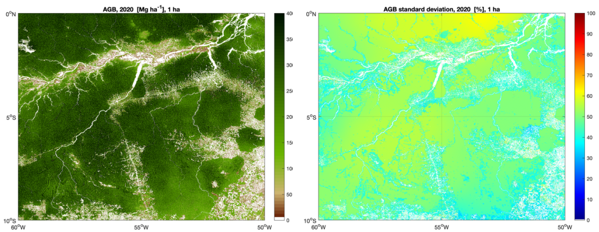
Figure 4-1: AGB (left) and AGB relative SD (right) for 2020. The colour ramps are constrained between 0 and 400 Mg ha -1 (AGB) and between 0% and 100% of the estimated AGB (AGB SD) to increase the colour contrast.
