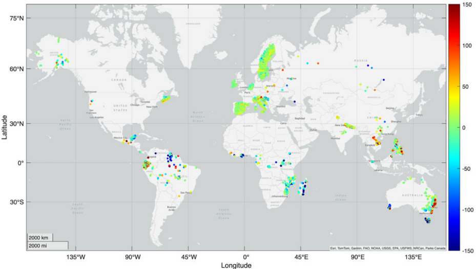
Figure 3-6: Map of the spatial distribution of estimation errors. Errors are defined as the difference between map-based and plot-based average AGB per grid cell. The colour bar is constrained between +/- 150 Mg ha -1 to enhance the contrast. The AGB differences are displayed for the 2010 dataset. The size of the circle is proportional to the number of field inventory measurements within a grid cell.
