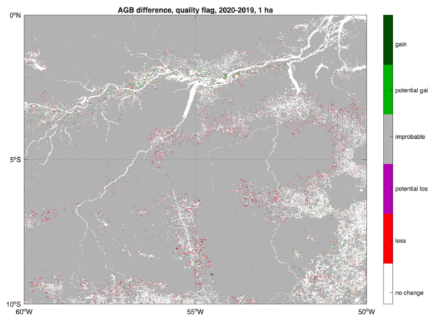
Figure 4-3: Quality flag of AGB change between 2019 and 2020.
