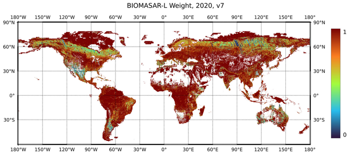
Figure 11-1: Map of the weight applied to estimates of AGB with the BIOMASAR-L approach in v7. Values closer to 1 indicate that the CCI BIOMASS AGB map is based primarily on the L-band estimate. Values closer to 0 indicate that the AGB map is based primarily on the C-band estimate.
