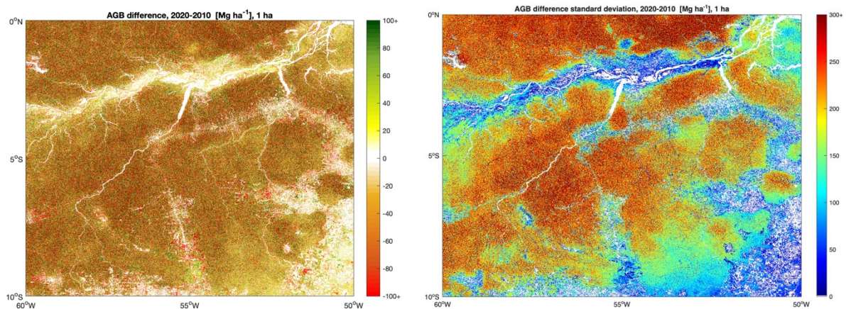
Figure 4-4: AGB change (left) and corresponding SD (right) between 2010 and 2020. AGB change is defined as difference between AGB maps of 2020 and 2010. The colour ramps are constrained between \pm 100 \text{ Mg ha}^{-1} (AGB change) and between 0 and 300 \text{ Mg} \cdot \text{ha}^{-1} (AGB change SD) to increase the colour contrast.
