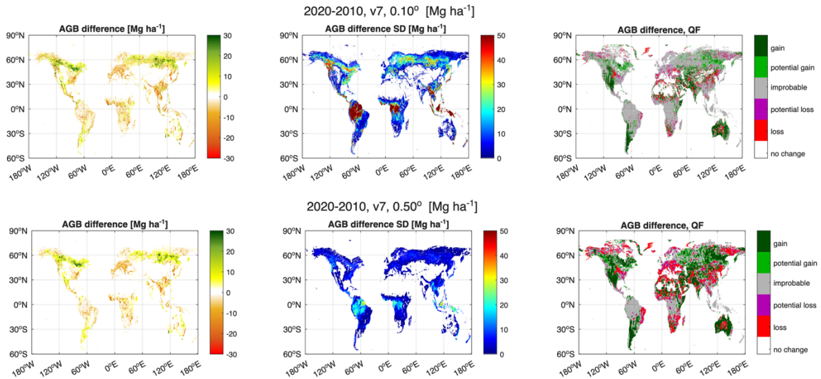
Figure 5-2: Maps of AGB change (left), corresponding standard deviation (middle) and quality flag (right) at 0.1° (top) and 0.5° (bottom) obtained by spatial averaging the CCI BIOMASS AGB maps of 2020 and 2010 and taking their difference.
