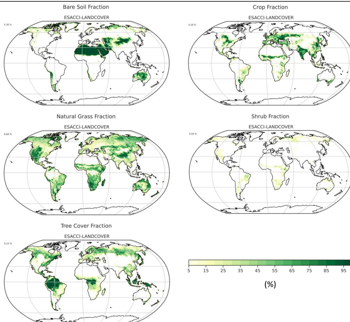
Figure 11 Example of the multi-year average (1992-2020) fractional coverage of (from top left to bottom right) bare soil, crops, natural grass, shrubs and trees from ESACCI LANDCOVER.
