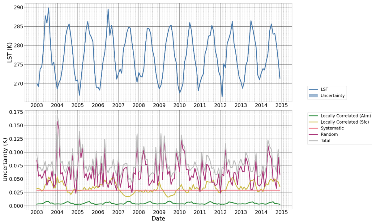
Figure 17 The same plots as in Figure 15 but for the night-time overpass data.
