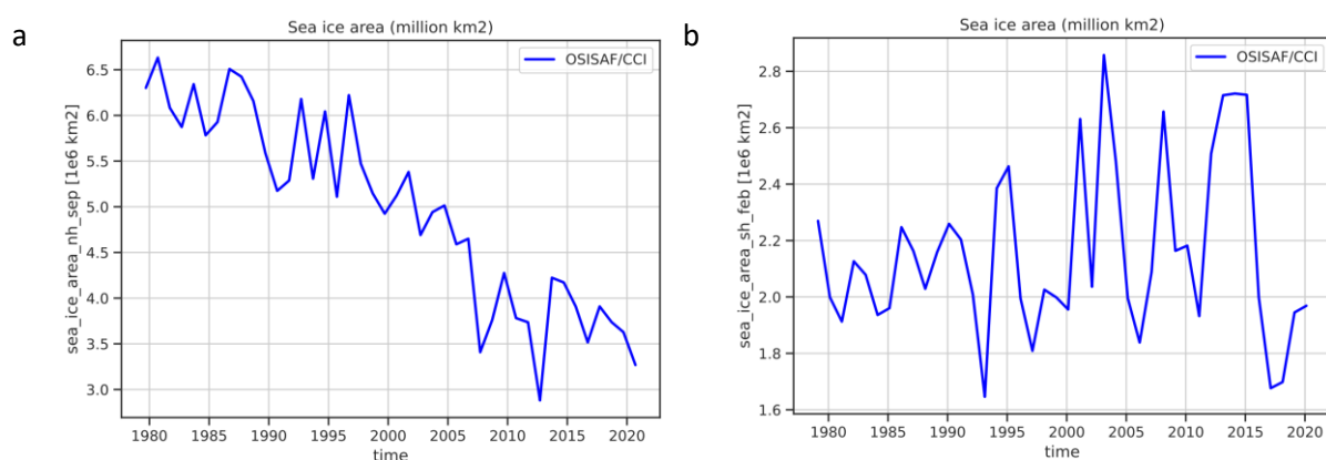
Figure 6 Time series of (a) Northern Hemisphere September sea ice area and (b) Southern Hemisphere February sea ice area in million km 2 from OSISAF/CCI SEA ICE. Sea ice area is calculated as the sum of the area size of all grid cells multiplied with its sea ice concentration.
