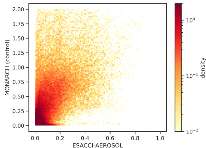
Figure 23 Example of processing output from the MONARCH model (BSC) with ESMValTool. Shown is a comparison of the simulated daily dust AOD at 550 nm (y-axis) with data from ESACCI AEROSOL (SLSTR) for June 2020.
