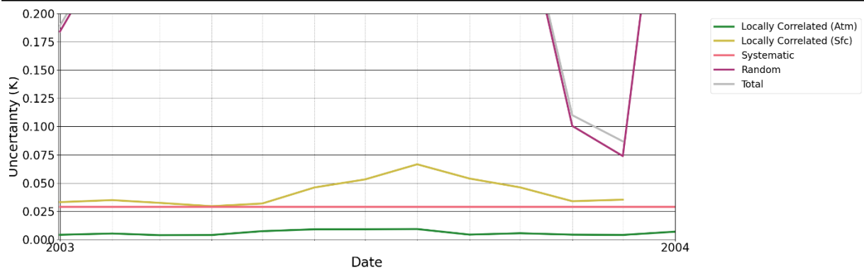
Figure 16 A zoom in on part of the daytime LST uncertainty values as propagated for the year 2003 and uncertainty values of less than 0.2 K. This shows the structure in both locally correlated components.
