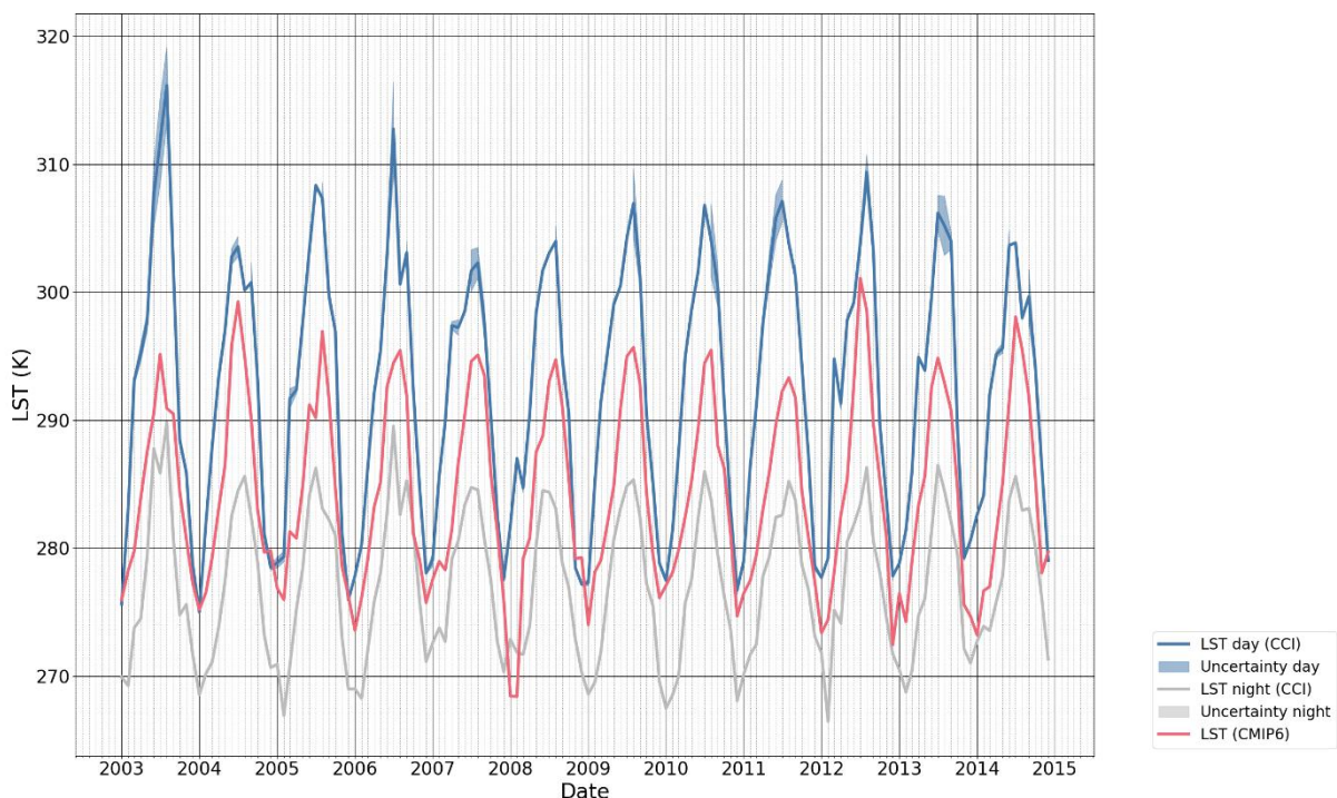
Figure 20 The LST_cci and calculated total uncertainty, and model comparison. The daytime and night-time overpasses from the LST_cci are given in blue and grey respectively, with shaded regions showing \pm 1 total uncertainty as in Figure 9. The red line is the land surface temperature from the model discussed in the text.
