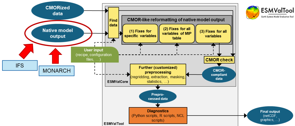
Figure 21 Schematic overview of the ESMValTool workflow from finding and correcting data to preprocessing and the scientific diagnostics.
