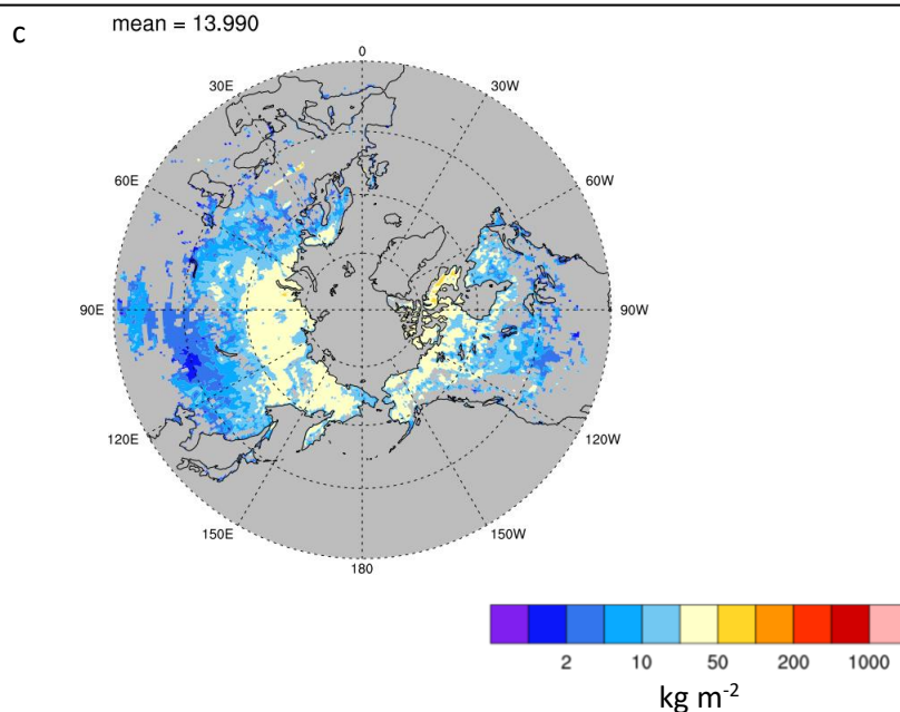
Figure 2 5-year average (2000-2004) seasonal mean surface snow amount (snow water equivalent, kg m -2 ) in the Northern Hemisphere (30°-90°N) from ESA CCI SNOW for (a) December-January-February (DJF), (b) March-April-May (MAM), (c) September-October-November (SON). There are no data available in June-July-August (JJA).
