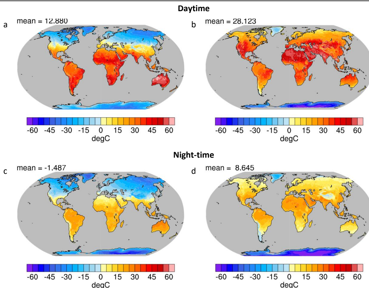
Figure 10 Multi-year (2003-2018) seasonal average land surface temperature (°C) from ESA CCI LAND SURFACE TEMPERATURE regrided to 0.5^{\circ} \times 0.5^{\circ} . (a) Daytime average for December-January-February, (b) daytime average for June-July-August, (c) night-time average for December-January-February, and (d) night-time average for June-July-August.
