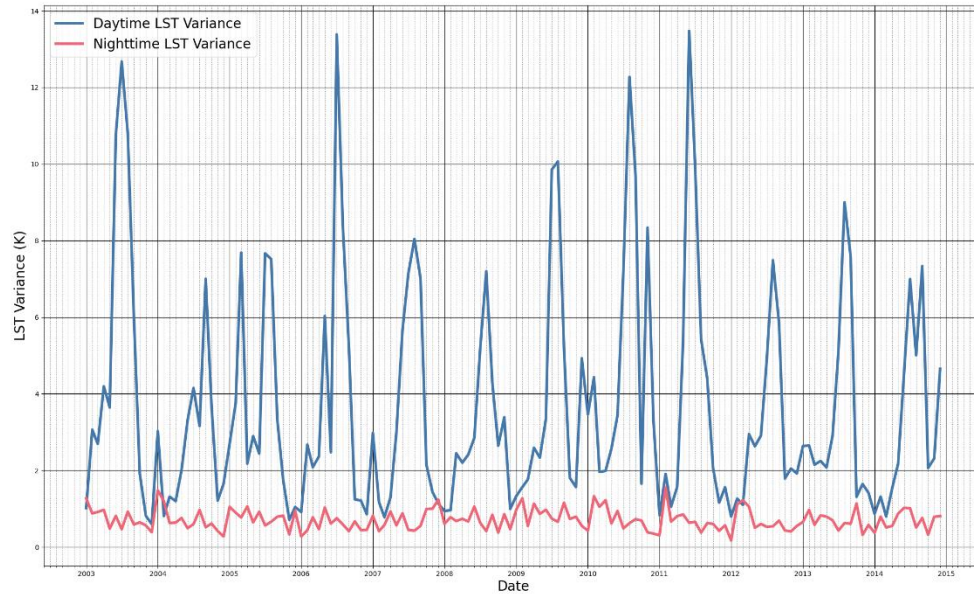
Figure 18 The land surface temperature (LST) variance of the daytime (blue) and night-time (red) overpasses for the region defined in the text. The daytime variance is seen to be large in the summer months. This affects the value of the propagated random uncertainty components at these times.
