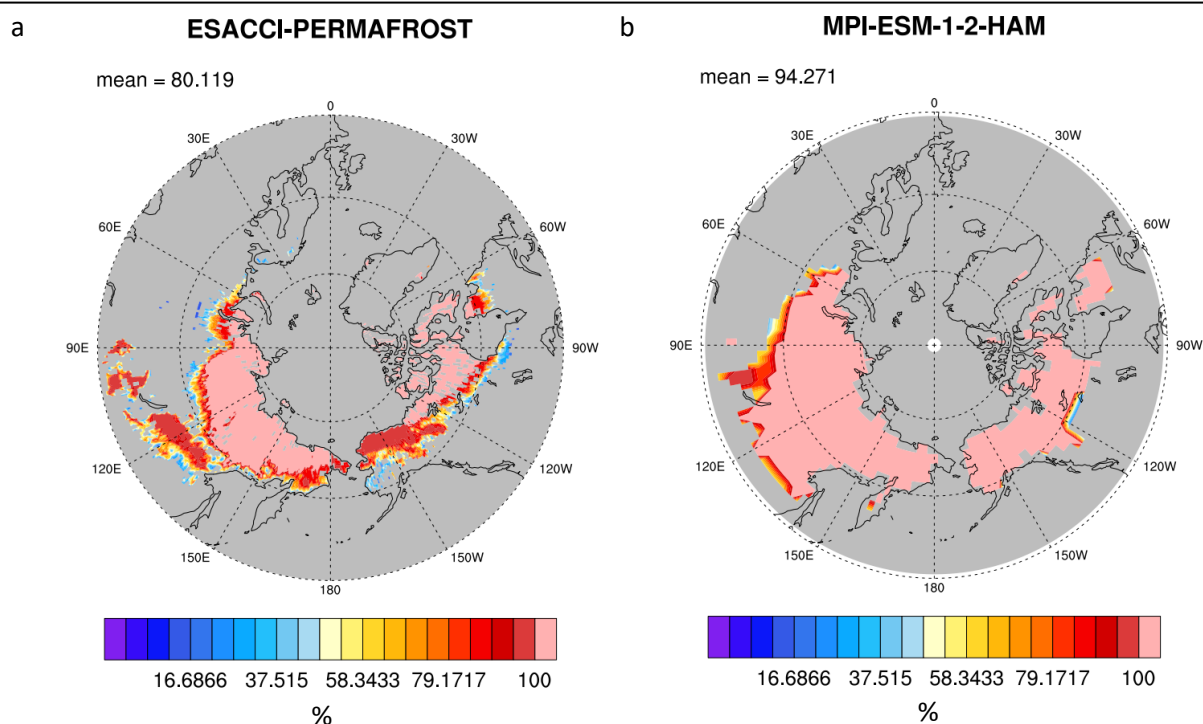
Figure 3 5-year average (2000-2004) permafrost extent (%) over ice-free regions in the Northern Hemisphere from (a) ESA CCI PERMAFROST compared with (b) the CMIP6 model MPI-ESM-1-2-HAM (historical simulation).
