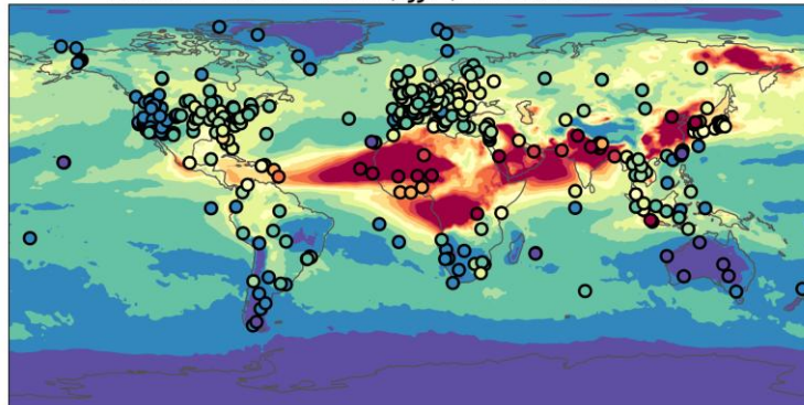
Total Aerosol Optical Depth at 0.44 microns Multi-Model-Mean, JJA, N stations=335
