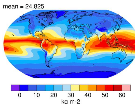
Figure 9 Multi-year (2003-2017) annual mean of the water vapor path ( \text{kg m}^{-2} ) from ESA CCI WATER VAPOUR.
