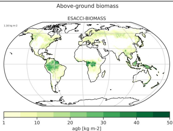
Figure 1 Annual mean above-ground biomass in \text{kg m}^{-2} from ESACCI-BIOMASS for the year 2022.
