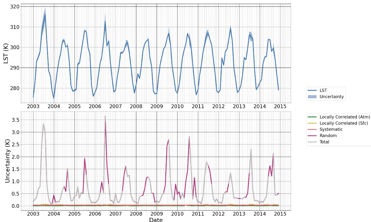
Figure 15 Timeseries plots of the daytime Land Surface Temperature (LST) and the propagated uncertainty components for the region of France defined in the text. (top) The mean LST shown with \pm 1 times the uncertainty shown as a shaded region. (bottom) The four uncertainty component values propagated across the region. The total combined uncertainty is given as the grey line.
