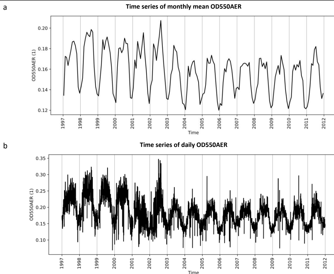
Figure 4 Time series of (a) monthly mean and (b) daily aerosol optical depth (AOD) at 550 nm averaged over the whole globe from SU_(A)ATSR v4.3.
