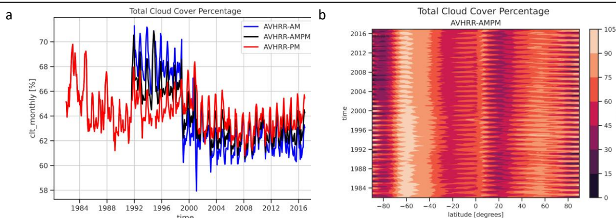
Figure 5 (a) Time series of global average monthly mean total cloud cover from ESACCI CLOUD AVHRR-AM (blue), AVHRR-PM (red) and the average over AVHRR-AM and AVHRR-PM (black). (b) Hovmoeller plot (latitude vs. time) of zonally averaged monthly mean total cloud cover averaged over AVHRR-AM and AVHRR-PM.
