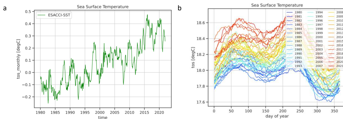
Figure 8 (a) Time series from 1980 to 2021 of global average monthly anomalies in sea surface temperature (reference period 1980-2009) from ESA CCI-SEA SURFACE TEMPERATURE. (b) Daily global mean sea surface temperature for each year in the time period 1980 to 2021 from ESA CCI SEA SURFACE TEMPERATURE.
