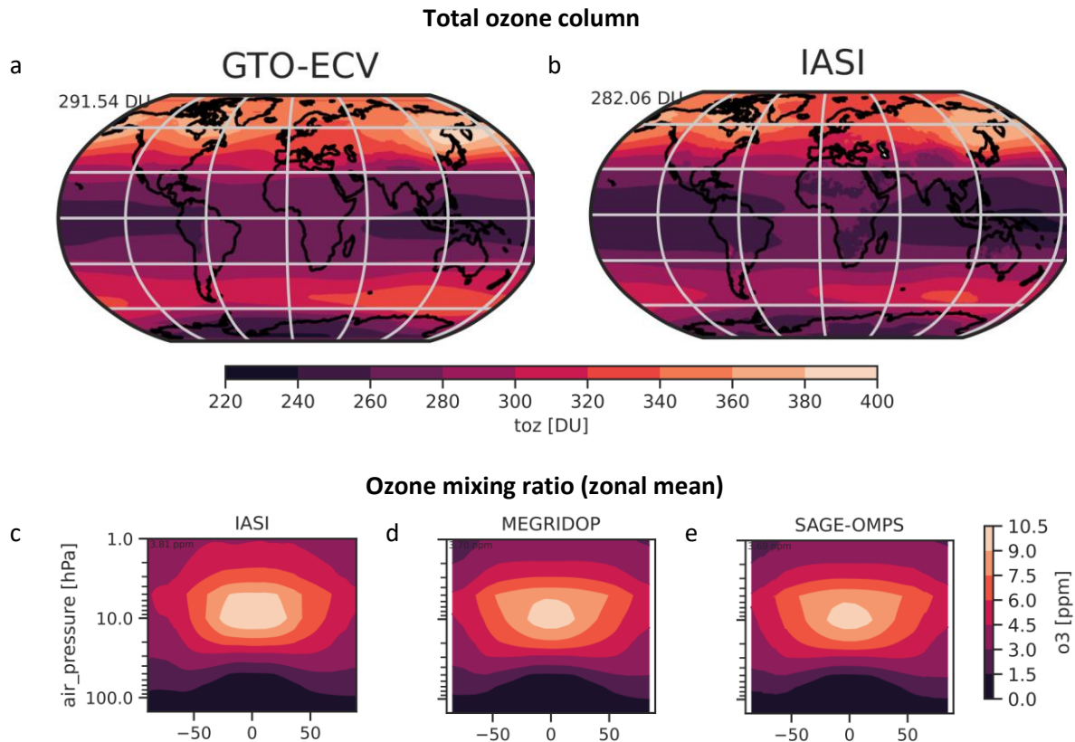
Figure 12 Multi-year (2008-2022) annual average (top) total column ozone in Dobson Units (DU) and ozone mixing ratio in ppm from ESA CCI OZONE. (a) GTO-ECV, (b, c) IASI, (d) MEGRIDOP, (e) SAGE-OMPS.
