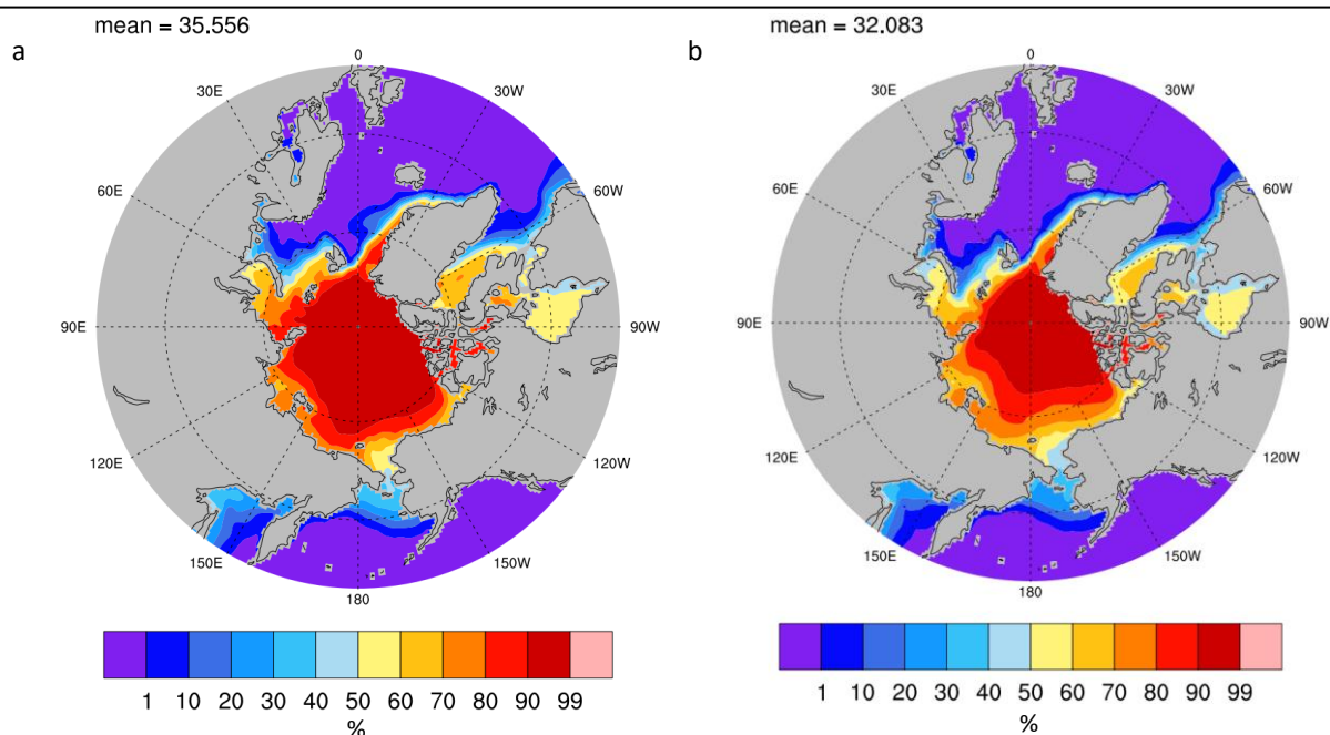
Figure 7 20-year annual average sea ice concentration in percent from OSISAF/CCI SEA ICE. (a) Average over 1980-1999, (b) 2000-2019.
