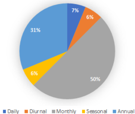
Figure 3: Permafrost_cci specific user requirements survey results for ground temperature temporal and spatial resolution (target)
