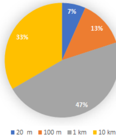
Figure 3: Permafrost_cci specific user requirements survey results for ground temperature temporal and spatial resolution (target)
