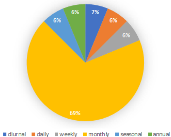
Figure 4: Permafrost_cci specific user requirements survey results for active layer thickness temporal and spatial resolution (target)
