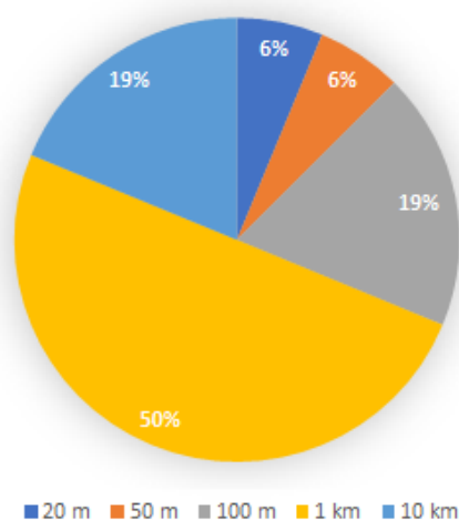
Figure 4: Permafrost_cci specific user requirements survey results for active layer thickness temporal and spatial resolution (target)
