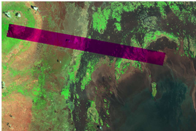
Figure 7 An example of a rare case of radiometric anomaly observed in Sentinel-2 MSI imagery of Lake Chilwa, 22 Nov 2018
