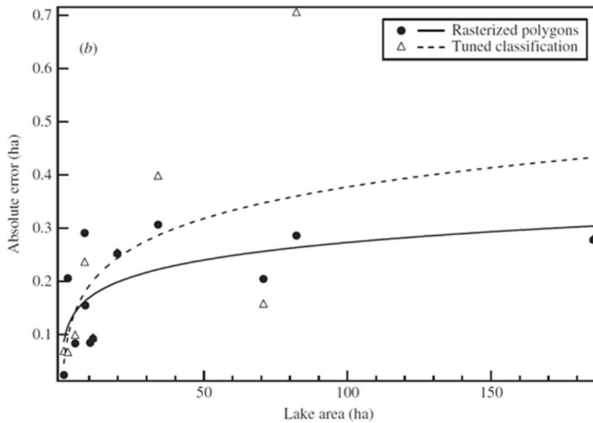
Figure 9 Scatter plots of absolute error in estimated lake area as a function of 'actual' lake area (based on DGPS shoreline measurements). Lines represent power-law fits to the respective data points (from Lyons et al. 2013)
