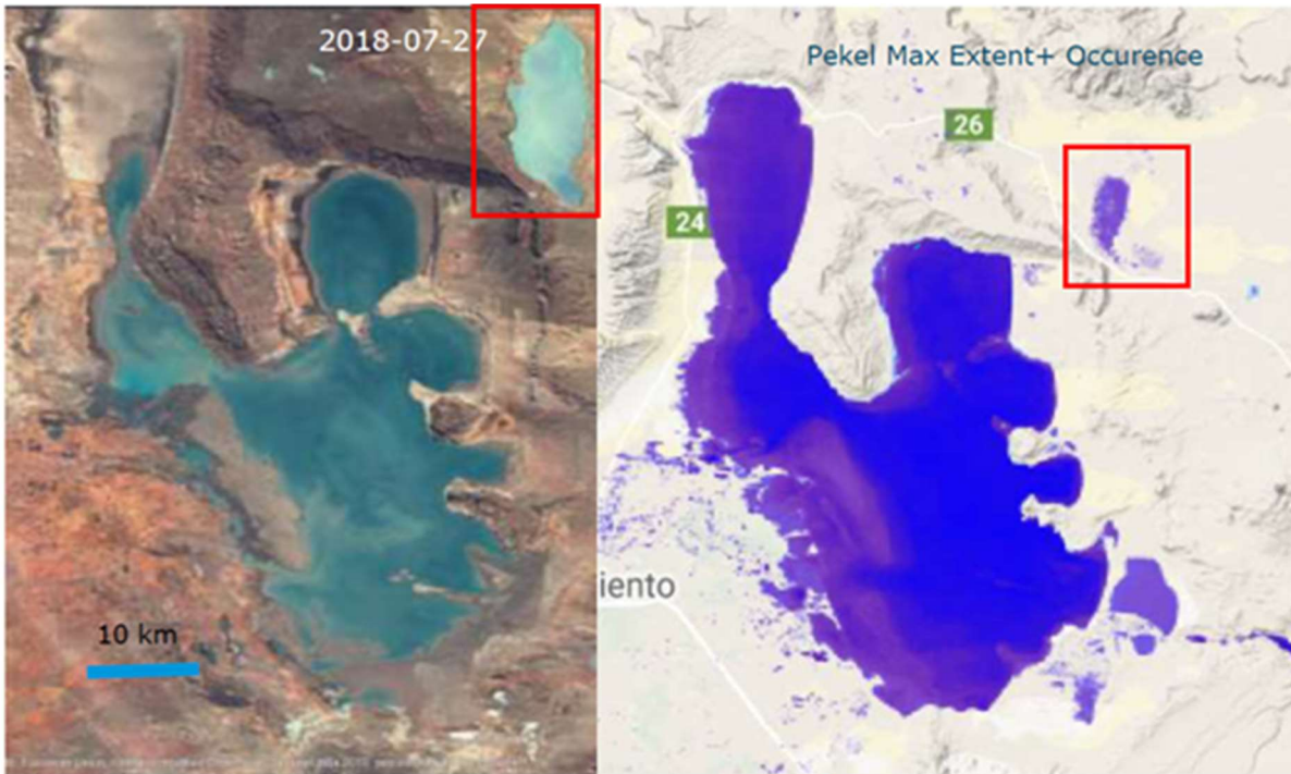
Figure 6 Lake Colhue (Argentina ) shows water despite pixels having 0% water occurrence in the GSW data set.
