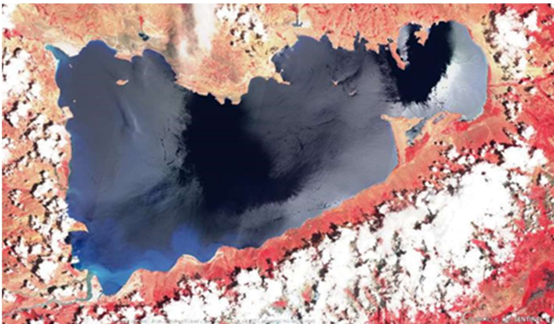
Figure 2 Sun glinted Sentinel-2 MSI image acquired on 14 Jul 2017 over Namtso lake (PR China)
