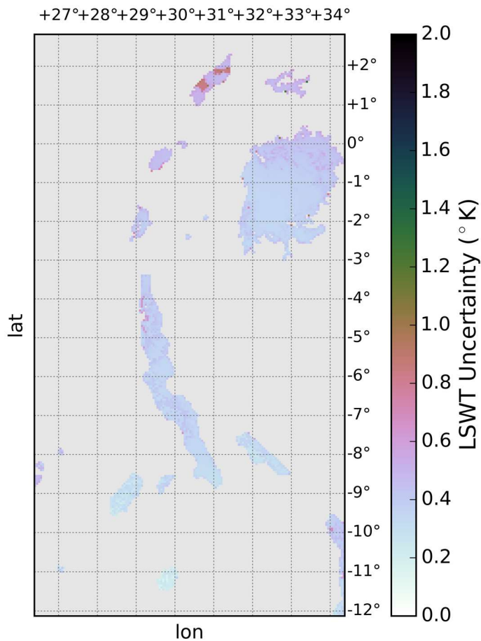
Figure 11 Uncertainty fields for L3 product for (top) Swedish lakes (the largest being Vanern and Vattern) and (lower) east African lakes (the largest being Lake Victoria).
