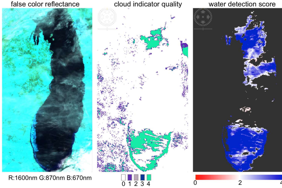
Figure 10 (Left) False colour composite image of reflectance at 1600 nm (R), 870 nm (G) and 670 nm (B). (Middle) the co-incident MERIS cloud indicator. (Right) The water detection score: QL 5 retrievals are made where this score reaches 4 or more. All panels for lake Michigan in USA on the 15-Feb-2011.
