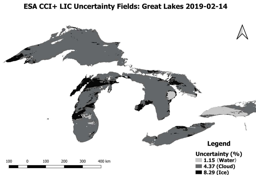
Figure 15. Uncertainty map of the Laurentian Great Lakes, Canada/USA, 14 February 2019.
