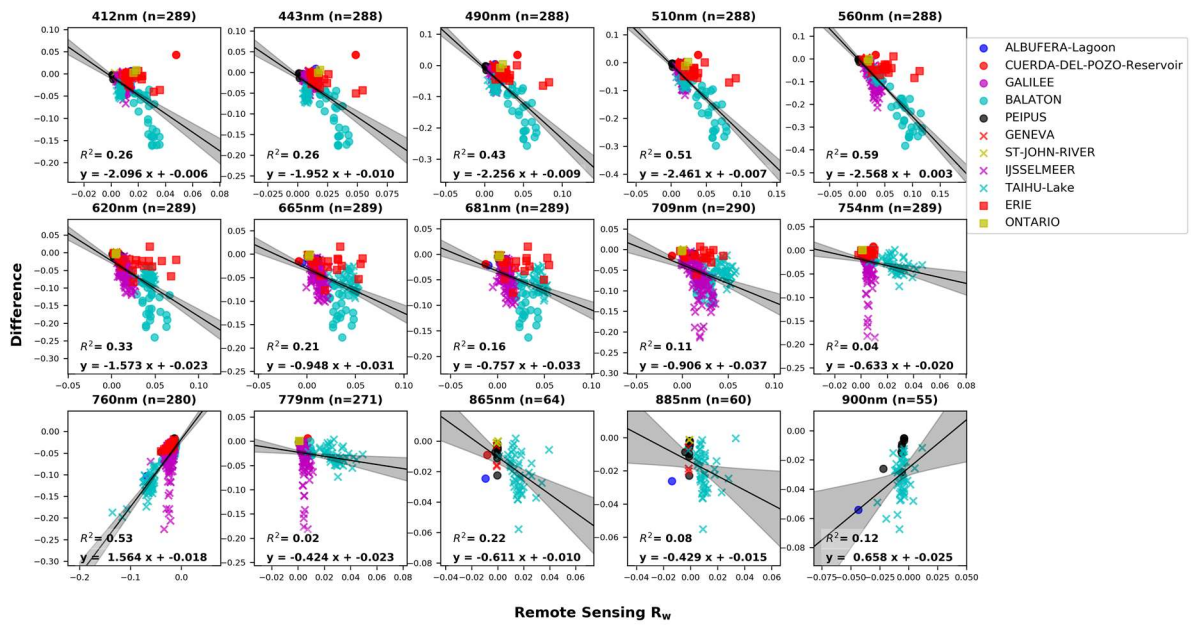
Figure 16 Linear correlation between Remote sensing R_w and the Difference between in situ and remote sensing R_w matchups (among which the wavebands of 865, 885 and 900 nm are not included in the R_w uncertainty products because of the sparse matchups).
