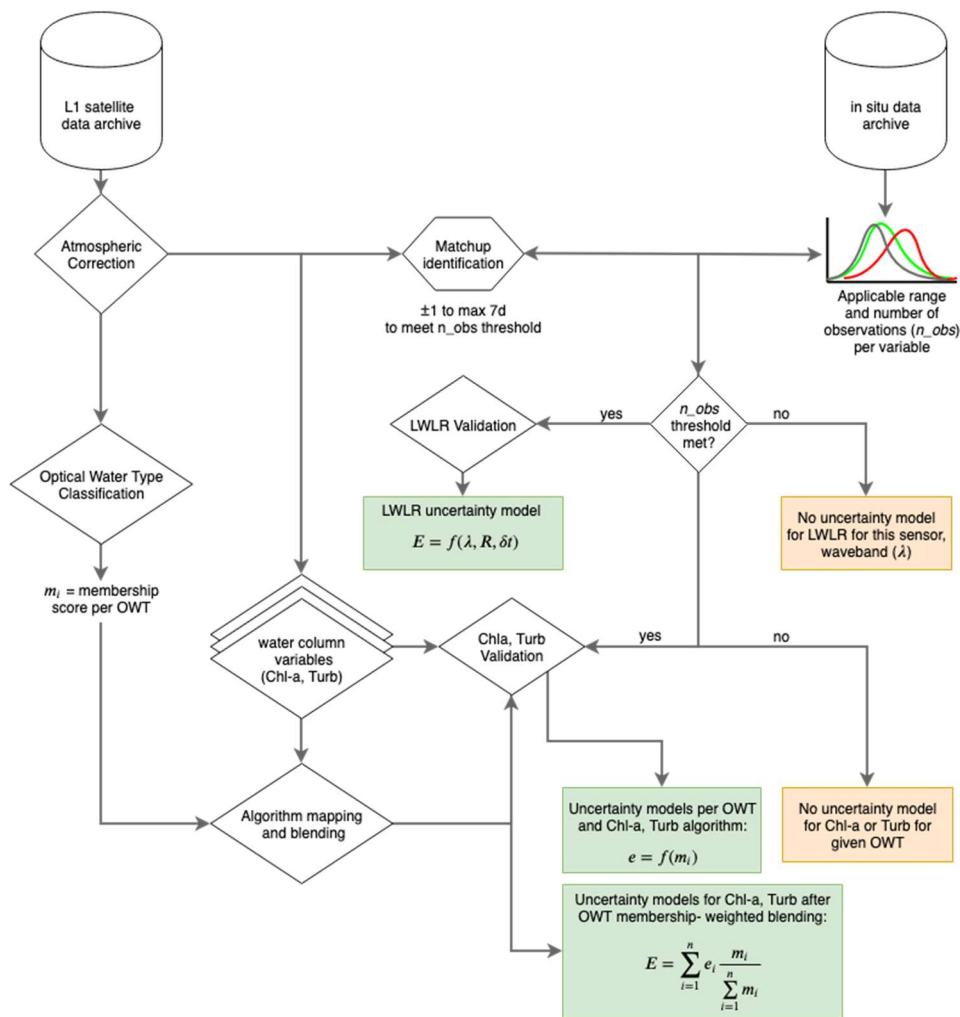
Figure 18 Flow chart of the end-to-end validation of LWLR products against in situ observations, resulting in uncertainty models.
