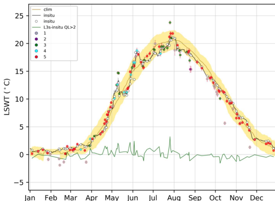
Figure 12 Satellite observations (dots), in situ matches (white dots), in situ measurements (black line), satellite minus in situ temperature difference for quality levels 3,4,5 (green line) and climatology (golden line) for lake Erken in Sweden in 2008.
