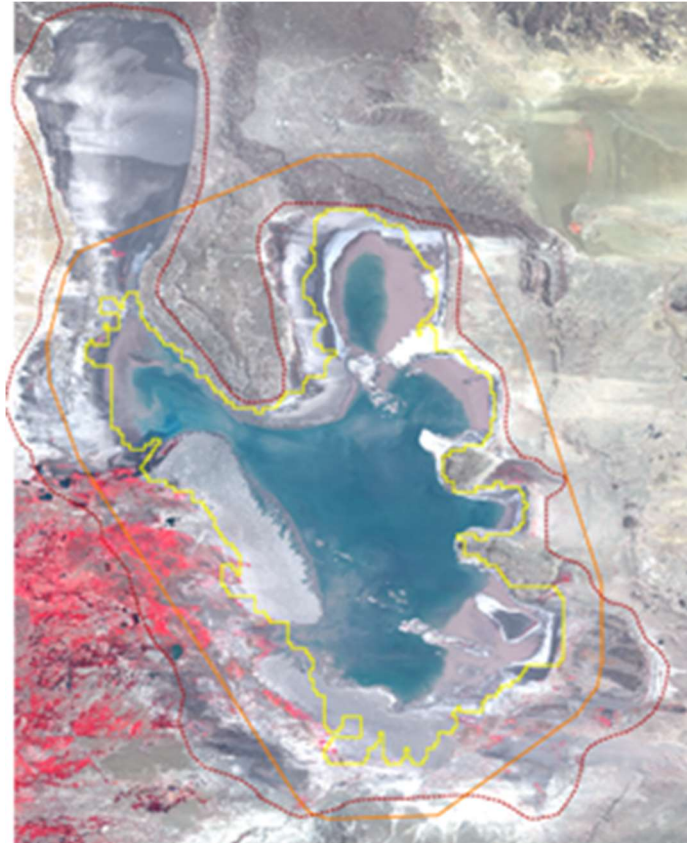
Figure 3 Reference envelope over Colhue Lake (Argentina). Yellow and orange (buffered) envelopes are derived from the ESA CCI Land Cover database and exclude the northern part of the lake. The red contour is based on high resolution satellite imagery.
