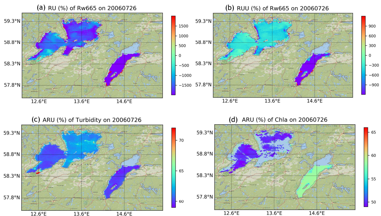
Figure 20 Per-pixel uncertainty products. (a) Relative uncertainty of R_w(665) , (b) Relative unbiased uncertainty of R_w(665) , (c) Absolute relative uncertainty of Turbidity and (d) Absolute relative uncertainty of chlorophyll- a .
