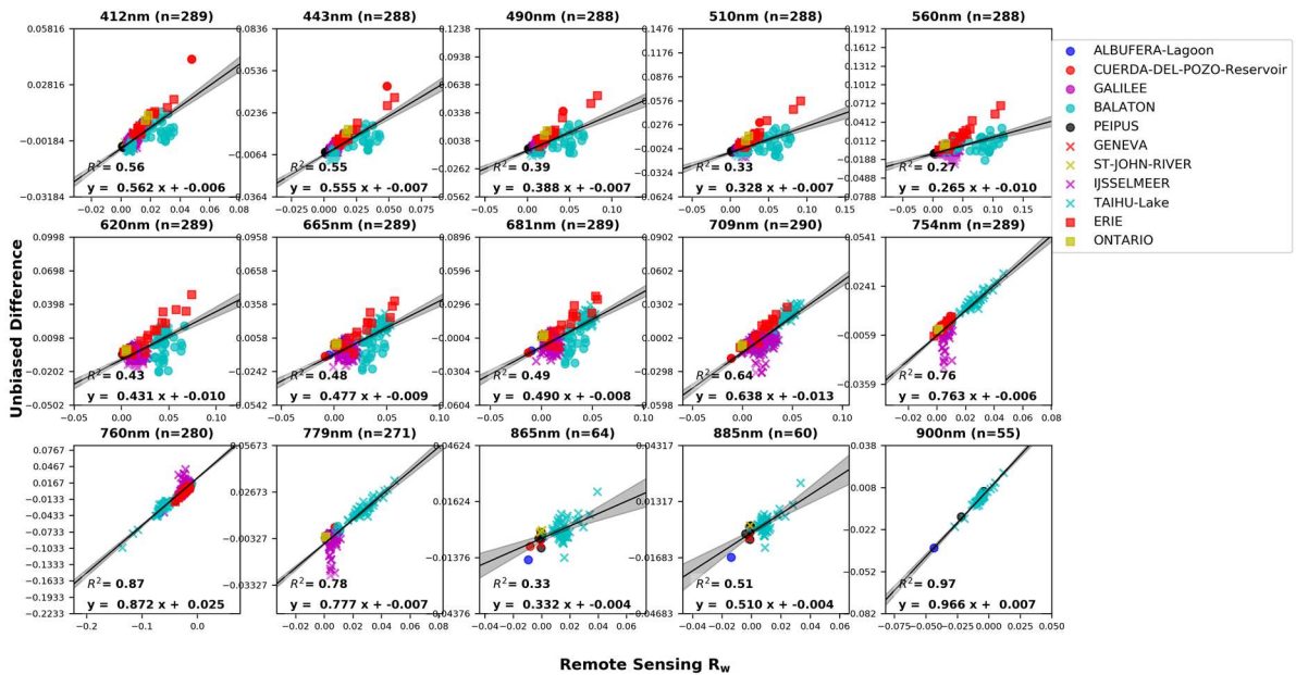
Figure 17 Linear correlation between Remote sensing R_w and the Unbiased Difference between in situ and remote sensing R_w matchups (among which the wavebands of 865, 885 and 900 nm are not included in the R_w uncertainty products because of the sparse matchups).
