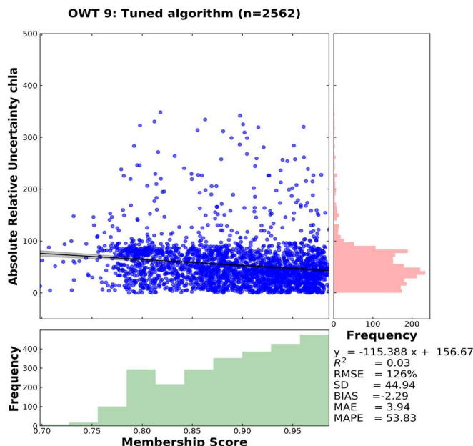
Figure 19 Correlation of Absolute Relative Uncertainty (ARU) of the top-3 weighted chlorophyll-a by the OWT membership score in relation to the membership score for optical water type 9. Reproduced from Liu et al. (in prep).
