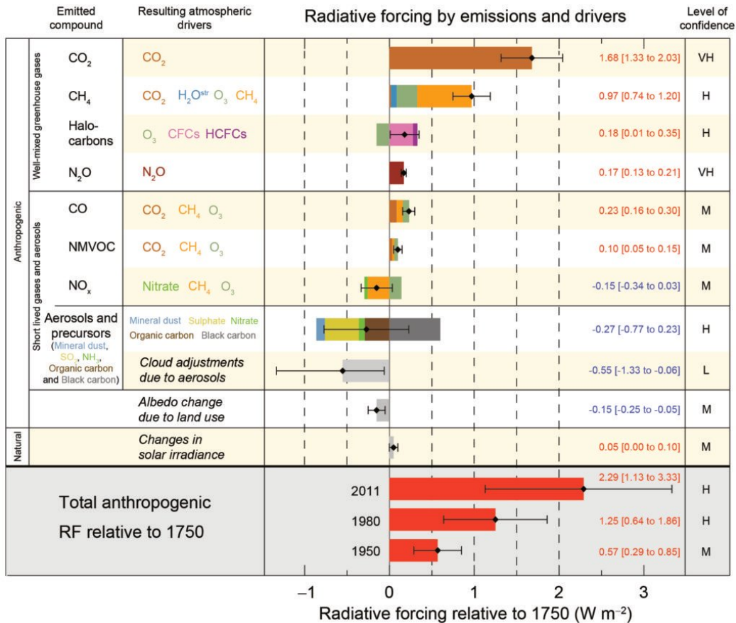
Figure 1: Radiative forcing estimates in 2011 relative to 1750 and aggregated uncertainties for the main drivers of climate change. Values are global average radiative forcing (RF14), partitioned according to the emitted compounds or processes that result in a combination of drivers. The best estimates of the net radiative forcing are shown as black diamonds with corresponding uncertainty intervals; the numerical values are provided on the right of the figure, together with the confidence level in the net forcing (VH – very high, H – high, M – medium, L – low, VL – very low). Albedo forcing due to black carbon on snow and ice is included in the black carbon aerosol bar. Small forcings due to contrails (0.05 W m -2 , including contrail induced cirrus), and HFCs, PFCs and SF 6 (total 0.03 W m -2 ) are not shown. Concentration-based RFs for gases can be obtained by summing the like-coloured bars. Volcanic forcing is not included as its episodic nature makes it difficult to compare to other forcing mechanisms. Total anthropogenic radiative forcing is provided for three different years relative to 1750. (Figure adapted from Figure SPM.5 of IPCC Fifth Assessment Report: Climate Change 2013: The Physical Science Basis)
