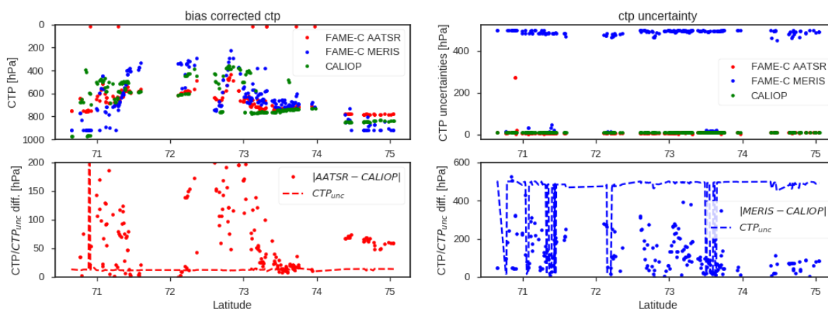
Figure 7-4 Case study 1 continued. Top-left: as Figure 7-3 but after bias removal. Top-right: CTP uncertainties; bottom-left: absolute difference of CTP_{AATSR} - CTP_{CALIOP} (after bias removal) and CTP_{AATSR,unc} ; bottom-right: absolute difference of CTP_{MERIS} - CTP_{CALIOP} (after bias removal) and CTP_{MERIS,unc} .
