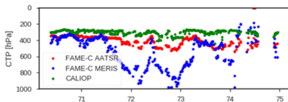
Figure 7-5 Case study 2. Comparison of CALIOP CTP with FAME-C CTP_{MERIS} and FAME-C CTP_{AATSR} .
