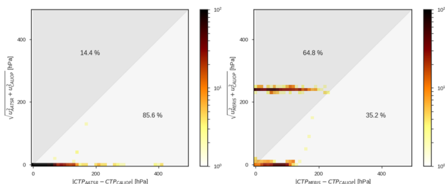
Figure 7-2 Two dimensional frequency histograms of FAME-C CTP_{AATSR} (left) and FAME-C CTP_{MERIS} (right) deviations from CALIOP (x-axes) compared to the combined uncertainties (y-axes). Also given are the relative numbers of cases for which the deviation is smaller than the combined uncertainty.
