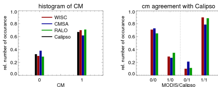
Figure 5-1 Comparison of MODIS cloud mask algorithms from CM SAF, WISC and RALOX algorithm with Calipso Cloud mask from the Product Validation and Algorithm Selection Report [R-7].
