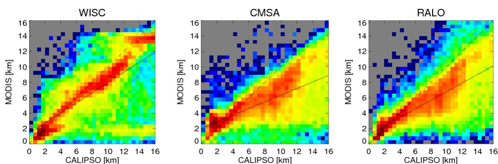
Figure 5-2 Comparison of MODIS Cloud top height retrievals from different algorithms with CALIPSO cloud height.
