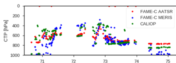
Figure 7-3 Case study 1. Comparison of CALIOP CTP with FAME-C CTP_{MERIS} and FAME-C CTP_{AATSR} .
