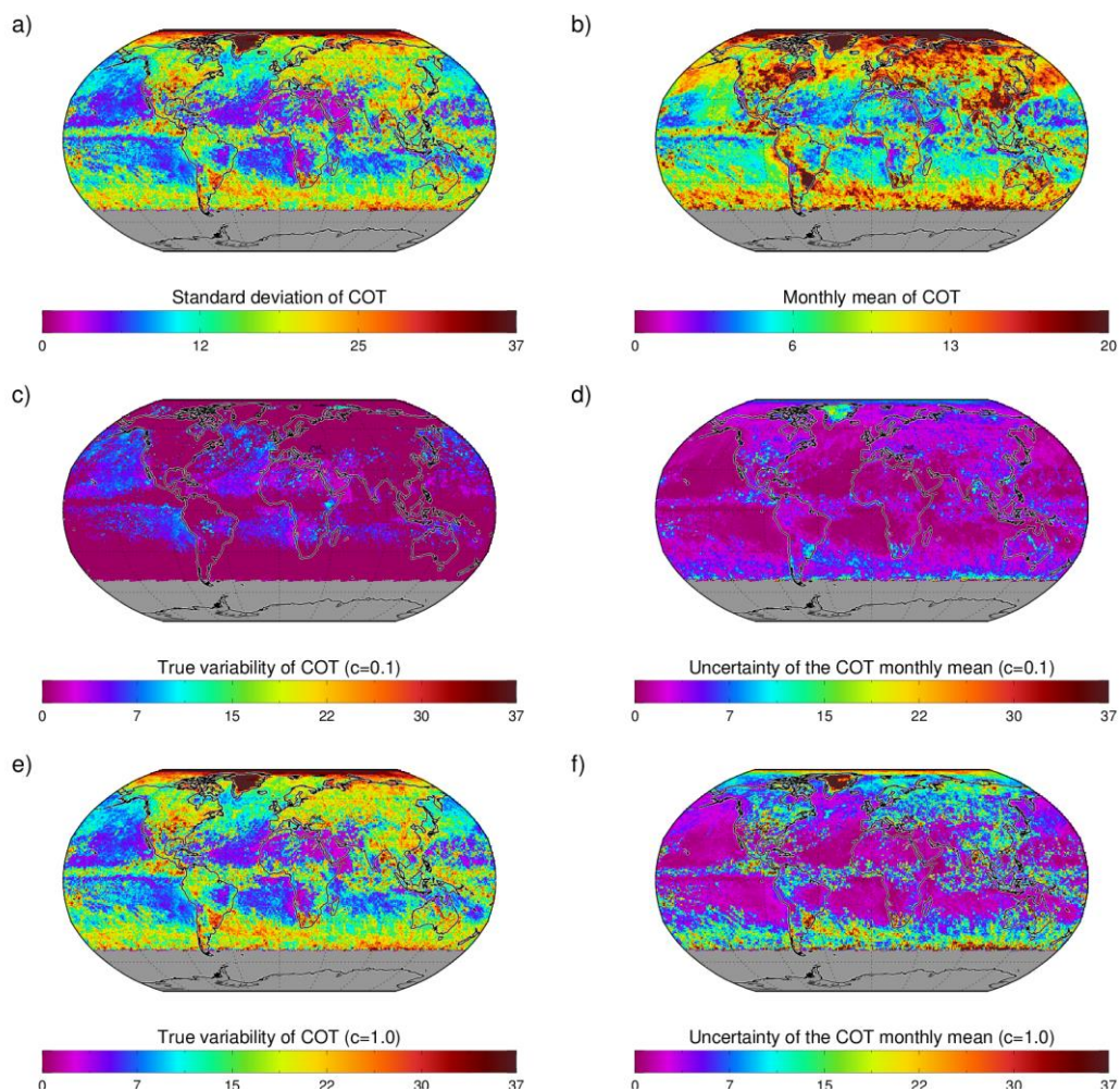
Figure 6-1 Monthly standard deviation (a) and monthly mean (b) for cloud optical thickness (COT). Panels (c) and (d) show the estimated natural variability and uncertainty of the mean (d) for a correlation of 0.1. Panel (e) and (f) are as panels (c) and (d) but for an uncertainty correlation of 1.0. All data is from AVHRR-PM in 2008/06. Figure taken from Stengel et al. (2017).
