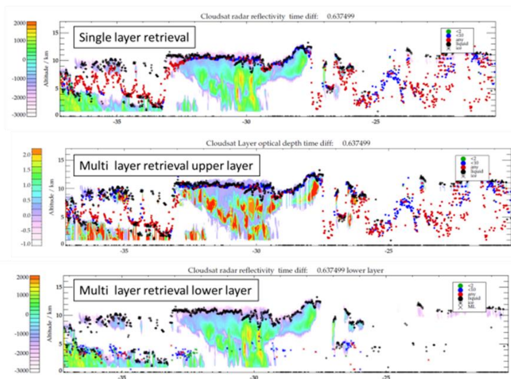
Figure 7-7 Shows a cross section of a MODIS multi-layer retrieval ( middle and lower panel) from 06/20/2008 compared with single layer retrieval (top panel). Collocated with coincident Cloudsat data. Red, blue green dots show the retrieved cloud top height, green dots have a low cost, red dots a high cost. Black dots show the actual cloud top height.
