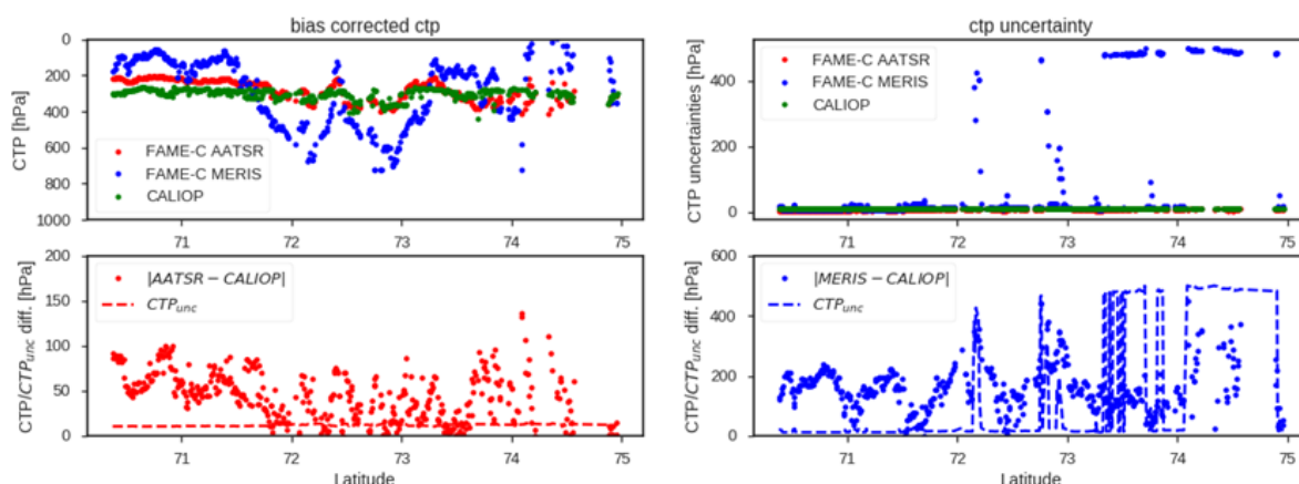
Figure 7-6 Case study 2 continued. Top-left: as Figure 7-5 but after bias removal. Top-right: CTP uncertainties; bottom-left: absolute difference of CTP_{AATSR} - CTP_{CALIOP} (after bias removal) and CTP_{AATSR,unc} ; bottom-right: absolute difference of CTP_{MERIS} - CTP_{CALIOP} (after bias removal) and CTP_{MERIS,unc} .
