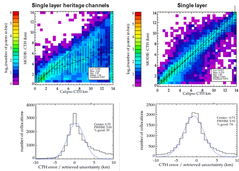
Figure 7-1 Shows a comparison of the upper layer cloud top height with Calipso (top) and the corresponding uncertainty validation (bottom) (Calipso - CC4CL MODIS)/retrieved uncertainty.. The two retrievals shown are the single layer retrieval algorithm for the heritage CC4CL retrieval which uses only 5 channels (left), and a multi-channel single layer retrieval from CC4CL (right).
