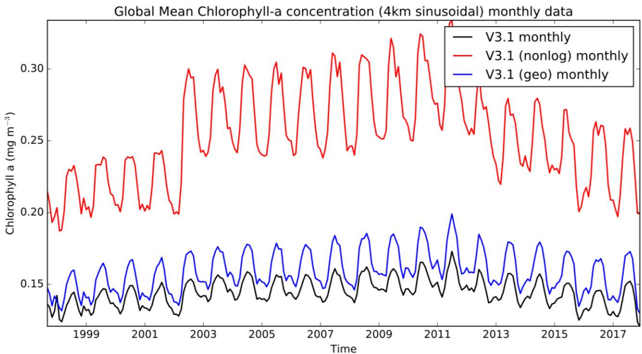
Figure 2: Comparison of Global mean Chlorophyll-a calculated using 1) the correct approach, \log(chl) from sinusoidal projection files (black line), 2) chl -a from geographic projection files (red line) and 3) \log(chl) from the geographic projection files.
