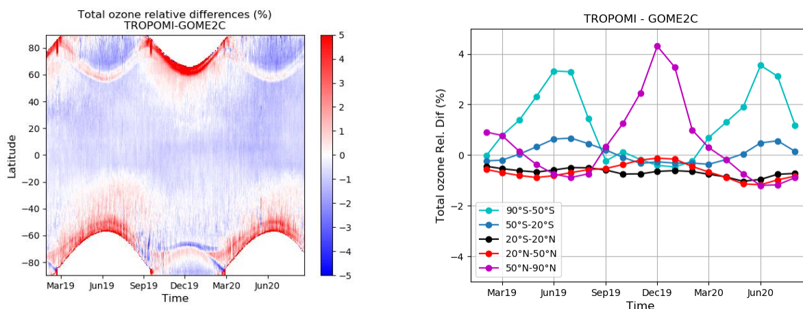
Figure 2-3: Comparison of the preliminary GOME-2C GODFITv4 total ozone product with the TROPOMI OFFL total product v01. The left panel shows mean relative differences as a function of time and latitude. The right panel shows the time dependence of mean differences in different latitude bands.
