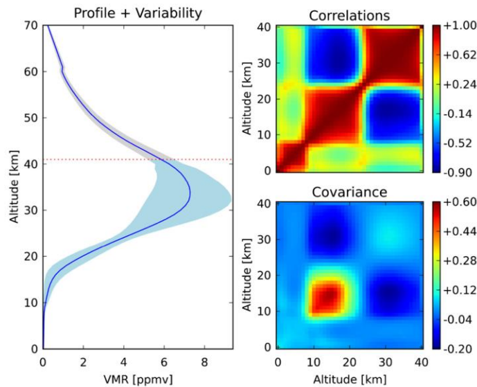
Figure 3-1. Left: x_a (ppmv, blue line) and associated variance (shaded blue) for the FORLI-O3. The dashed red line indicates the top altitude of the last retrieved layer. Right: correlations and \mathbf{S}_a variance–covariance matrices in unitless multiplicative factor. (from Hurtmans et al. 2012)
