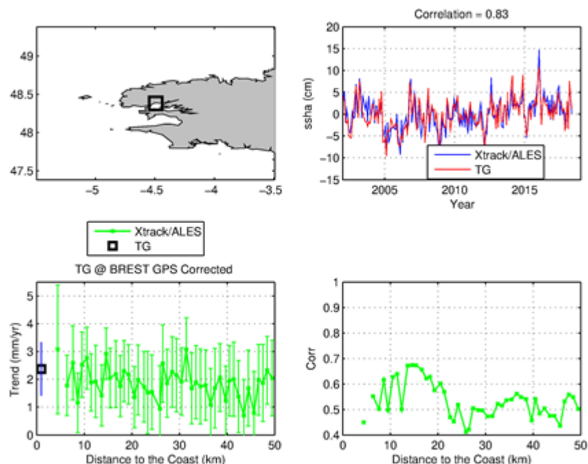
Figure 12: Validation at the Brest tide gauge. Map showing location of the tide gauge (top left), ‘best’ deseasoned monthly altimetry timeseries (see Section 3.3) compared with the monthly tide gauge record (top right), trend as a function of distance to the coast (bottom left), and correlation as a function of distance to the coast (bottom right).
