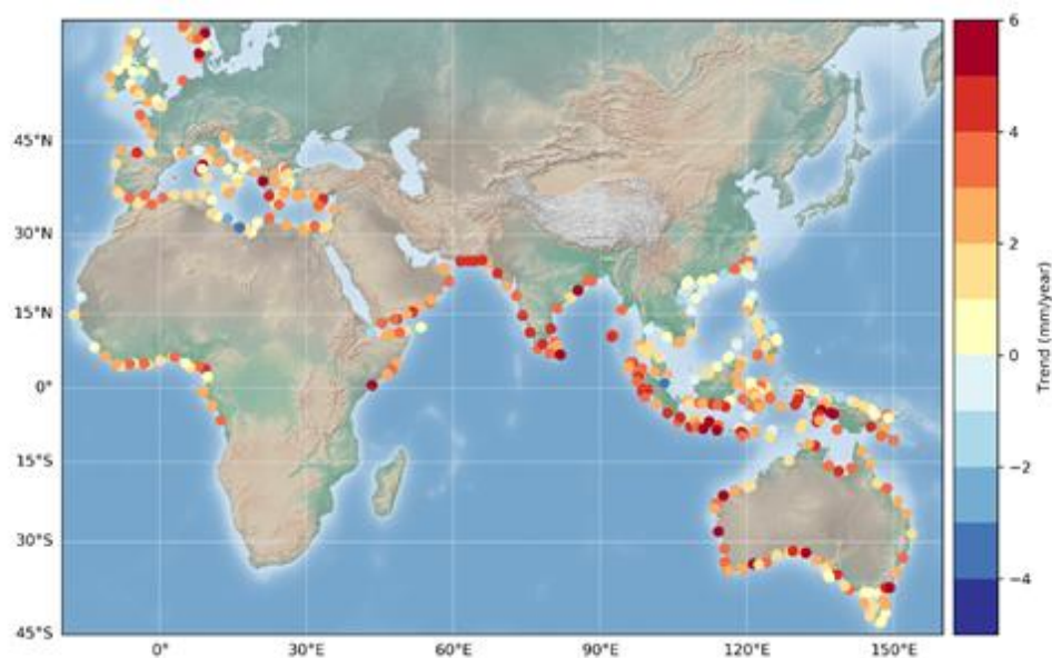
Figure 3. Coastal sea level trends (mm/yr) at the first valid point from the coast at the 429 selected sites.
