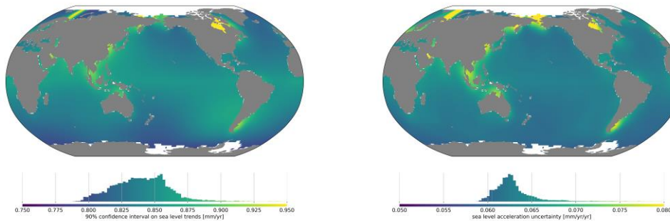
Figure 18, 90% confidence interval on regional sea level trends (left) and accelerations (right)
