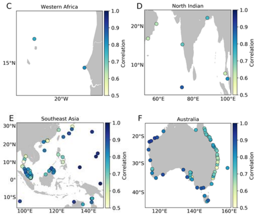
Figure 8: Correlation of detrended, deseasoned sea level from tide gauge records and satellite altimetry (the ‘best’ timeseries computed as described in Section 3.3) in (A) the Northeast Atlantic Ocean, (B) the Mediterranean Sea, (C) the Western African coast, (D) the North Indian Ocean, (E) Southeast Asian, and (F) Australia.
