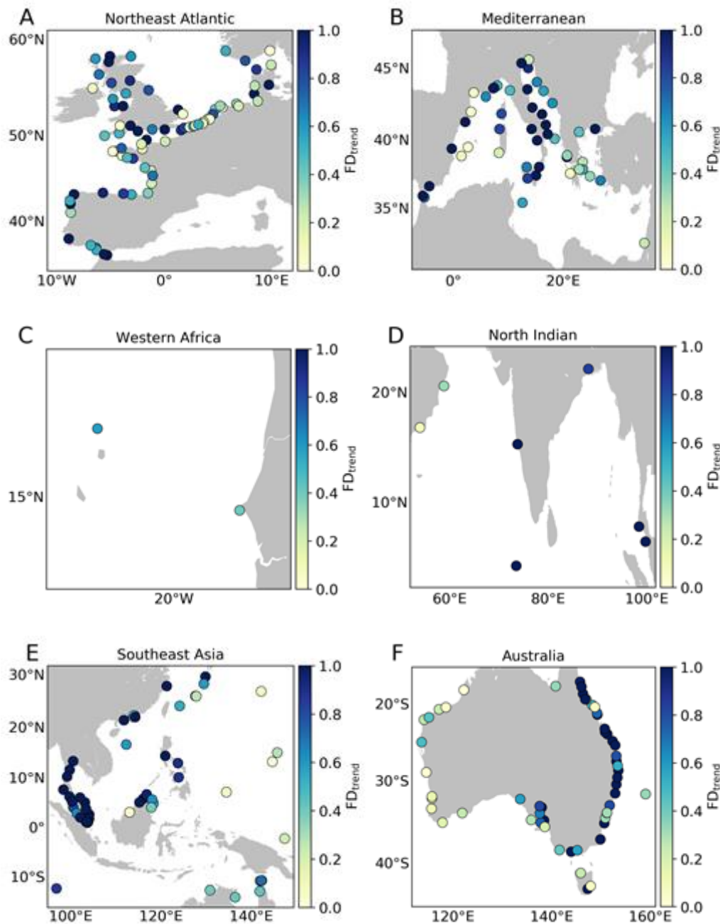
Figure 11: FDs between the sea-level trends from tide gauge records and from satellite altimetry (the ‘best’ timeseries computed as described in Section 3.3) over the period from January 2002 to May 2018 in (A) the Northeast Atlantic Ocean, (B) the Mediterranean Sea, (C) the Western African coast, (D) the North Indian Ocean, (E) Southeast Asian, and (F) Australia. Note that the colorbar has been saturated for the sake of clarity (i.e., the range of FDs is not limited to the range from 0 to 1).
