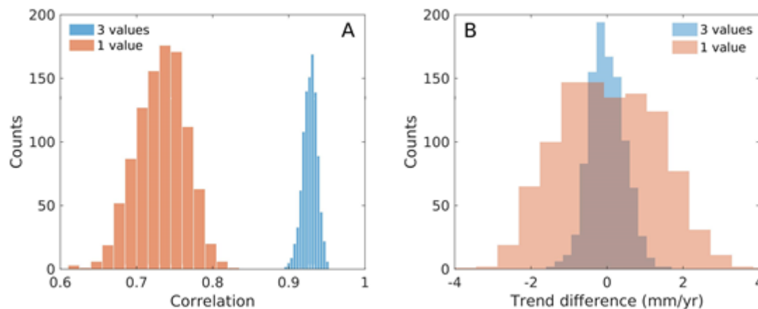
Figure 7: (A) correlation of 3-value and 1-value monthly timeseries with the true monthly means. (B) Difference in trend estimates from 3-value and 1-value monthly timeseries relative to the trend from the true monthly means.
