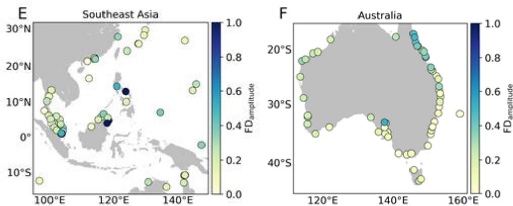
Figure 10: FDs between the amplitude of the sea-level annual cycle from tide gauge records and from satellite altimetry (the ‘best’ timeseries computed as described in Section 3.3) in (A) the Northeast Atlantic Ocean, (B) the Mediterranean Sea, (C) the Western African coast, (D) the North Indian Ocean, (E) Southeast Asian, and (F) Australia.
