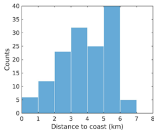
Figure 9: Histogram showing the closest distance to coast where the correlation between the tide gauge and altimetry data remains consistent with the correlation at more distant locations.
