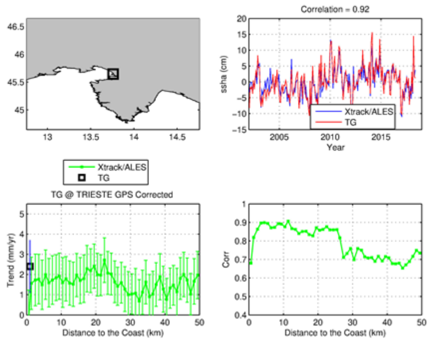
Figure 13: Same as Figure 12 but for the Trieste tide gauge.
