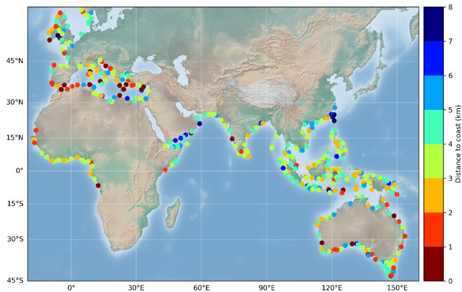
Figure 4: Map of the closest distance (km) to the coast of the first valid point from the coast at the 429 selected sites.
