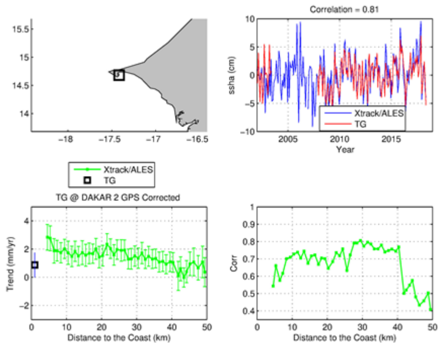
Figure 14. Same as Figure 12 but for the Dakar tide gauge.
