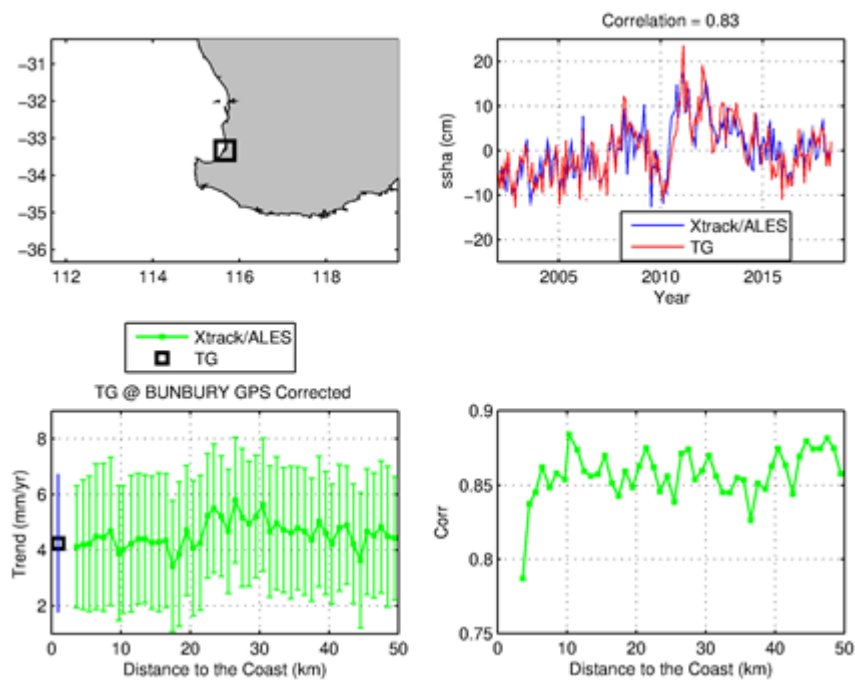
Figure 17: Same as Figure 12 but for the Bunbury tide gauge.
