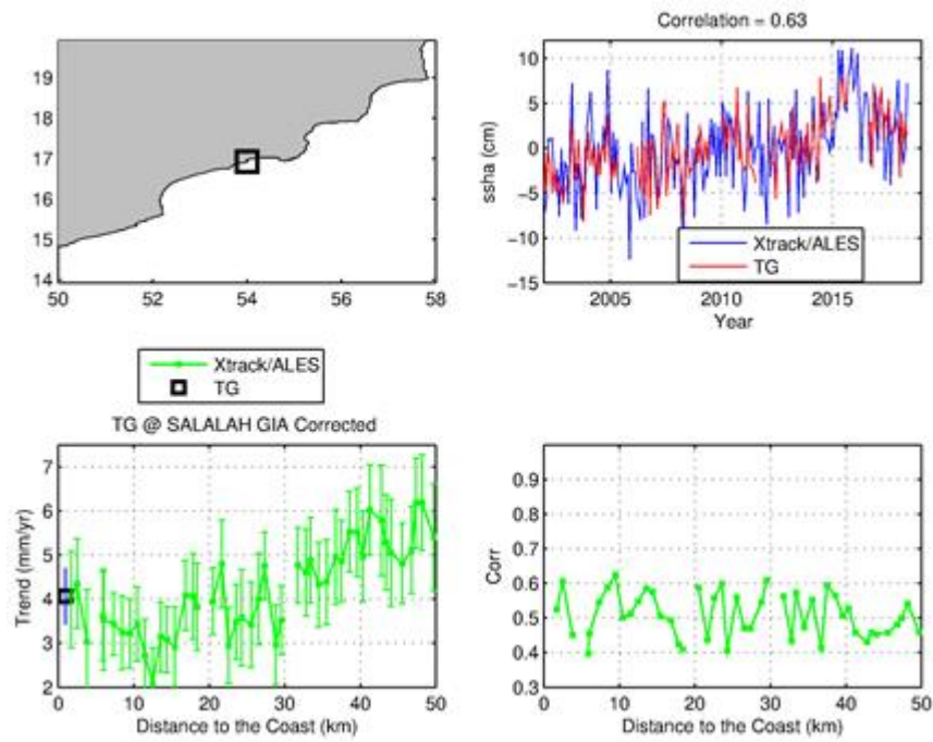
Figure 15: Same as Figure 12 but for the Salalah tide gauge.
