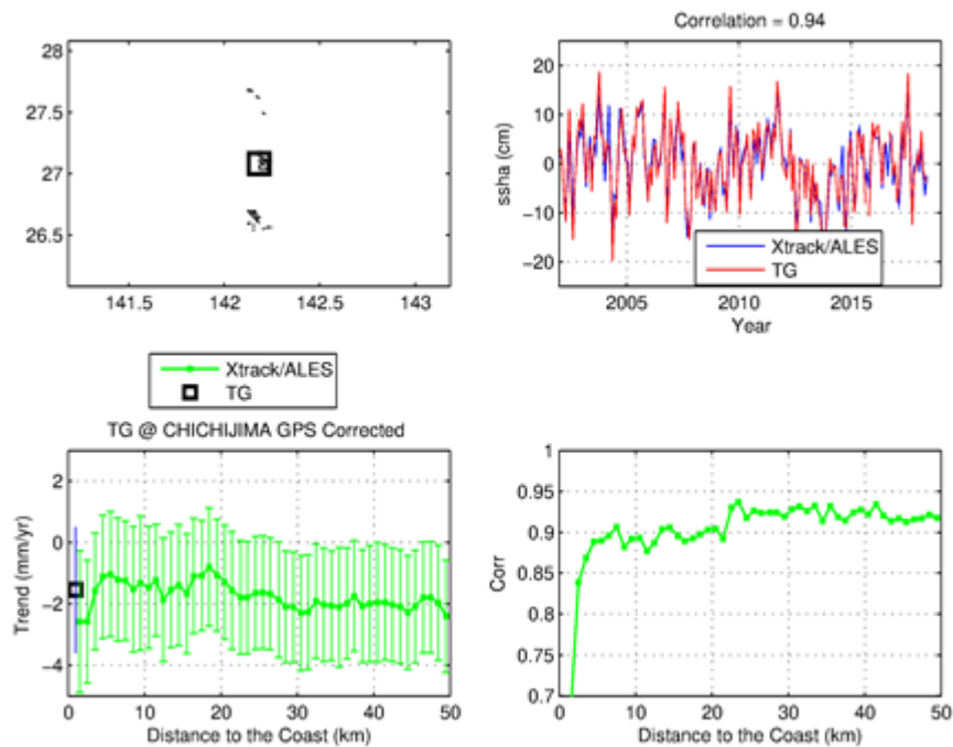
Figure 16: Same as Figure 12 but for the Chichijima tide gauge.
