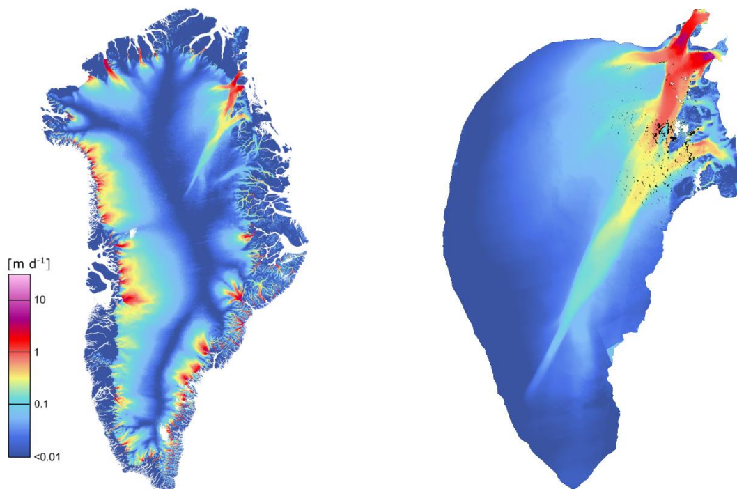
Figure 3.1: Left) Ice velocity map of the Greenland Ice Sheet based on Sentinel-1 data acquired during the 2019/20 winter mapping campaign from December 14 2019 to January 31 2020. Right: InSAR/offset-tracking map of Zwally Basin 2.1 between 2019-12-16 and 2020-01-25 from Sentinel-1.
