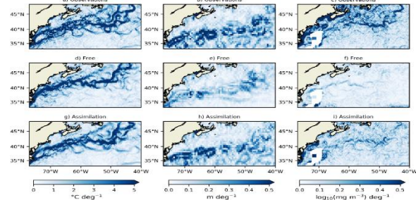
Figure 3: Impact on simulating Gulf Stream features from the assimilation of 4 ECV datasets.
